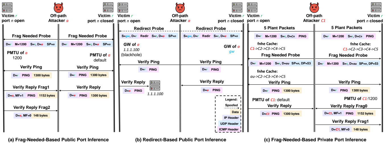
Keys: D=Destination IP, S=Source IP, M=PMTU, SP=Source Port, DP=Destination Port, MF=More Fragment, Cn(C1-C5)=Colliding IPs, au=Authoritative Name Server
