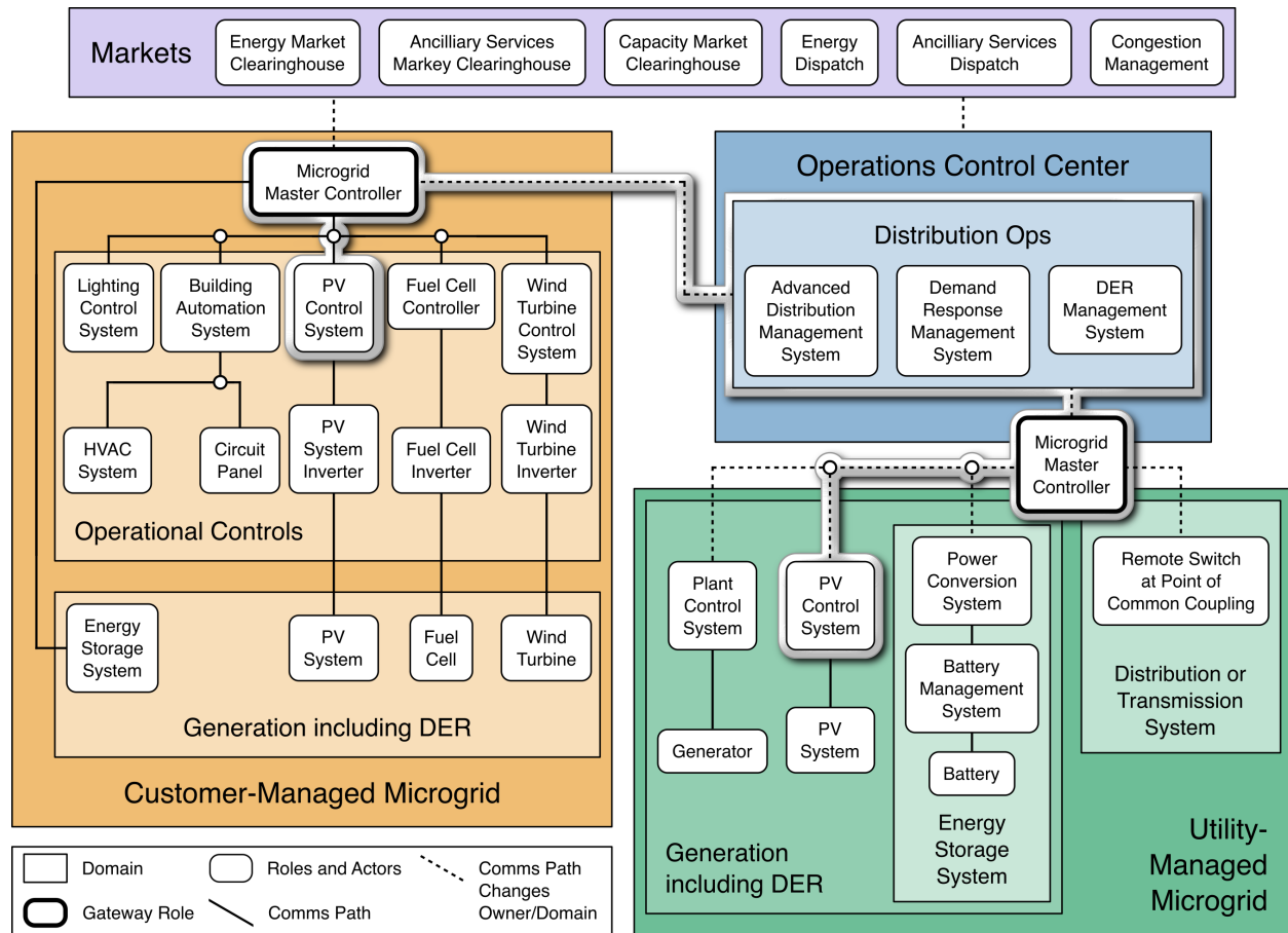
464 Figure 1 Microgrid Communications Pathways Scenario
