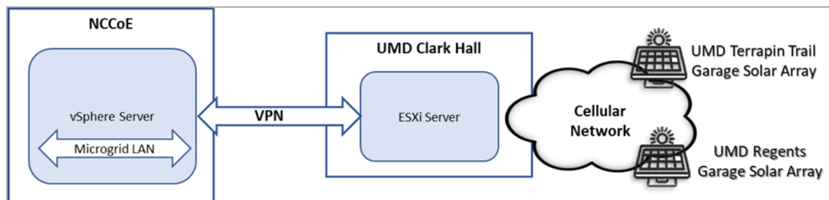
Figure 1-4 Overview of Laboratory Infrastructure
