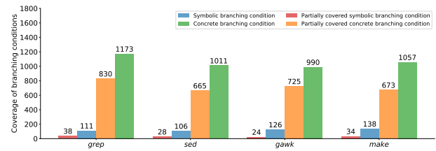
Figure 3: Coverage of different branching conditions.
