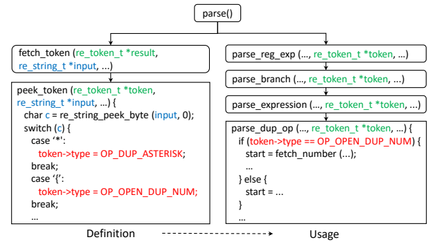
Figure 1: Function call chains for parsing inputs in grep 3.6 .
