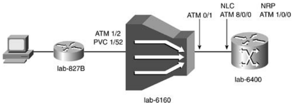
Figure 8-10. RBE Scenario
