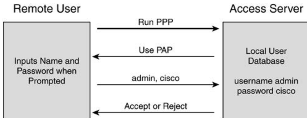
Figure 5-3. PAP Authentication
