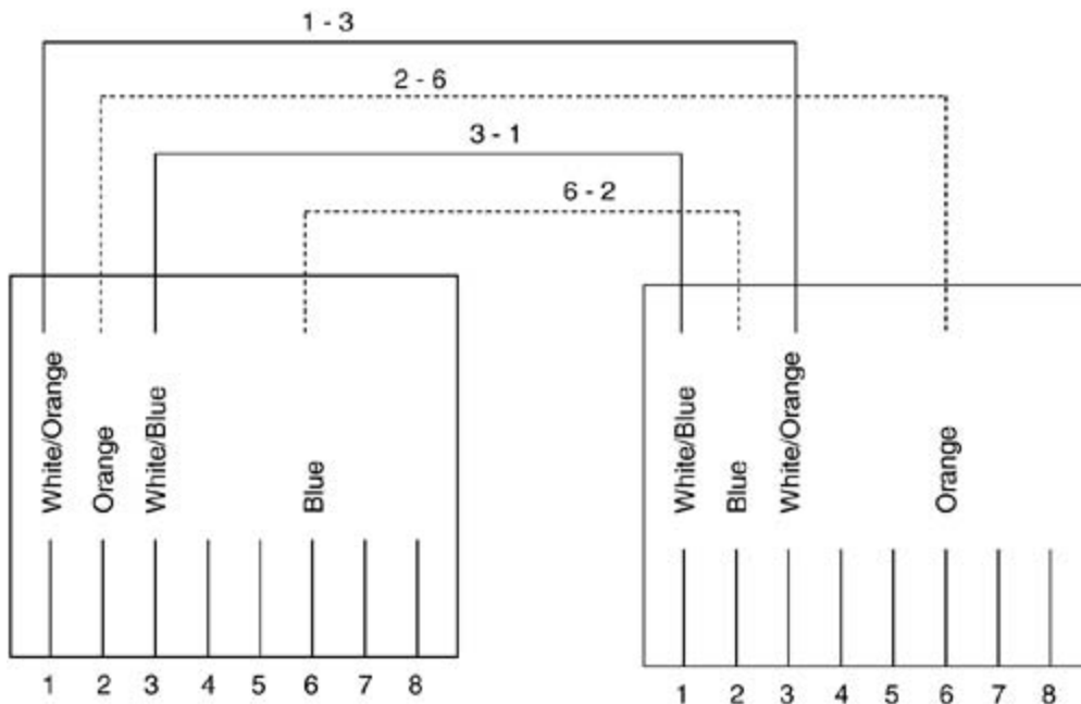
Figure 2-2. Pinouts for an Ethernet Crossover Cable
