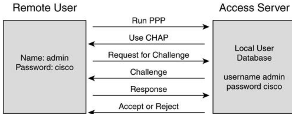
Figure 5-4. CHAP Authentication
