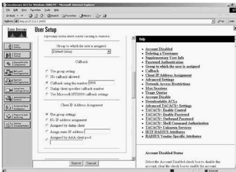
Figure 13-4. Cisco Secure ACS Configuration for ISDN Callback
