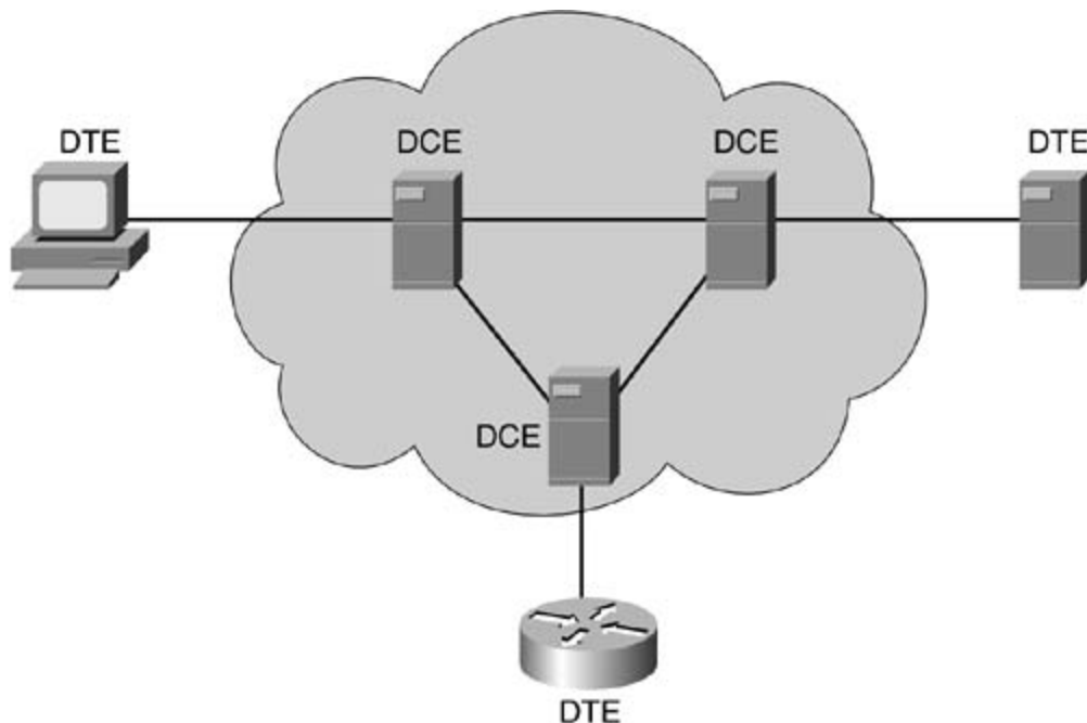
Figure 9-2. DTE / DCE Relationship
