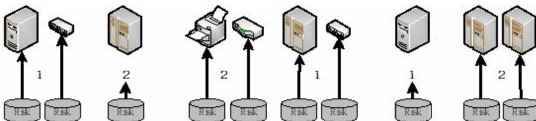
Figure 31: Asset Vulnerabilities
