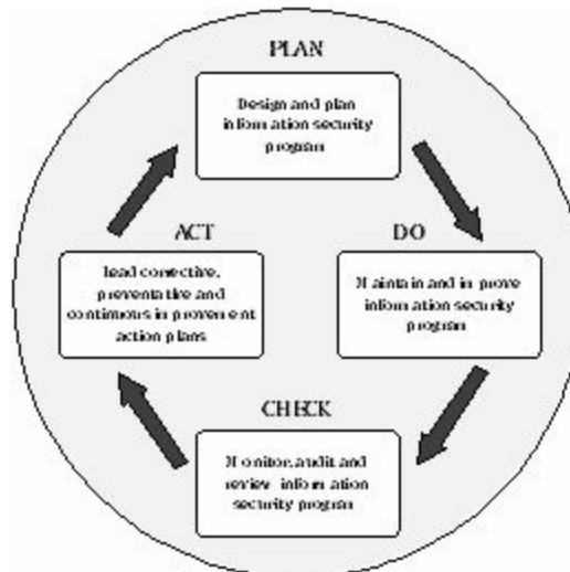
Figure 36: PDCA Methodology
