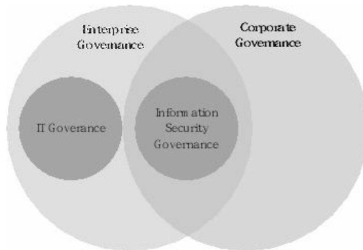
Figure 22: Governance Relationships
