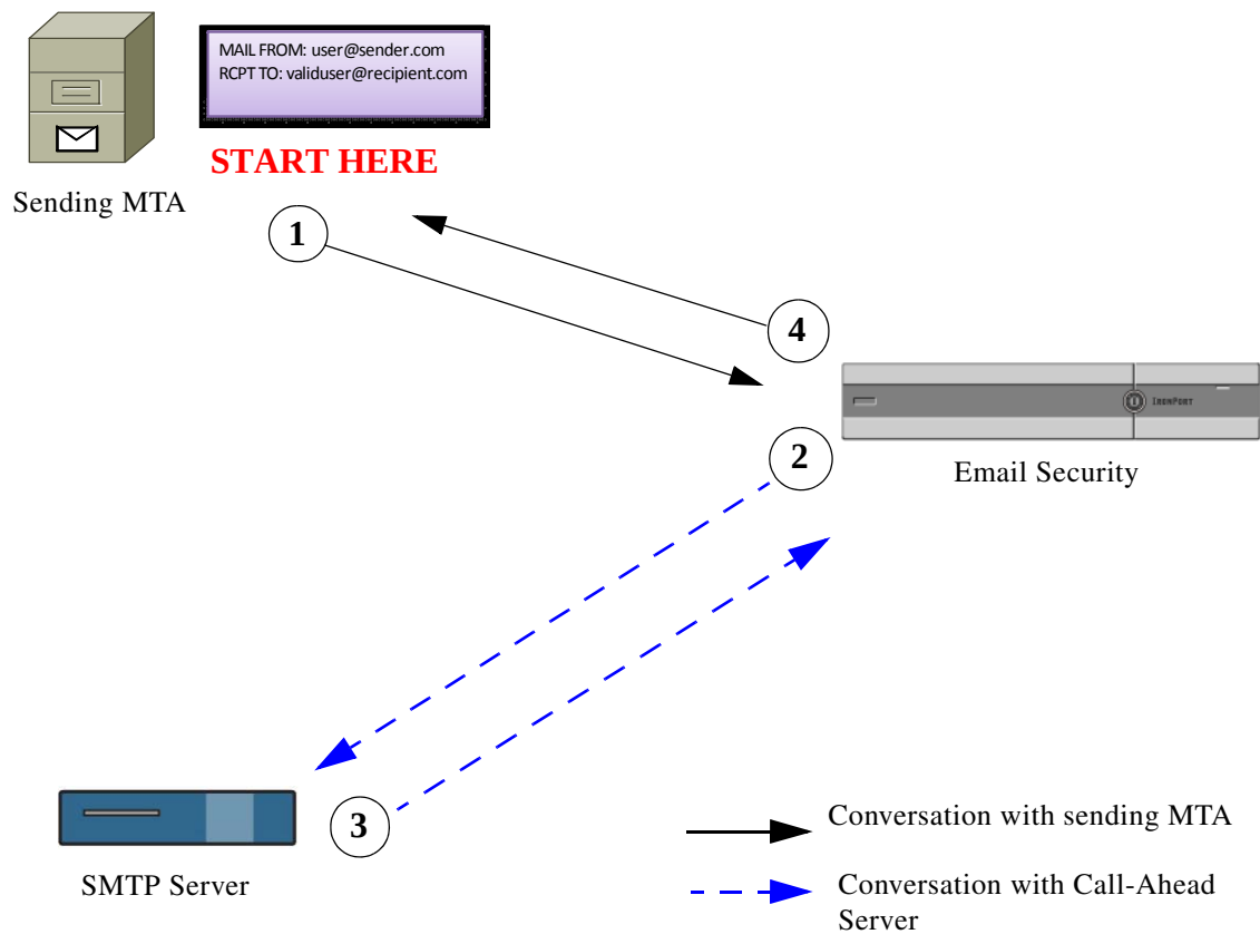
Figure 22-1 SMTP Call Ahead Server Conversation Workflow
