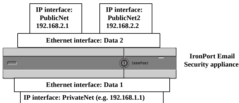
Figure 24-12 Adding Another Public Interface
