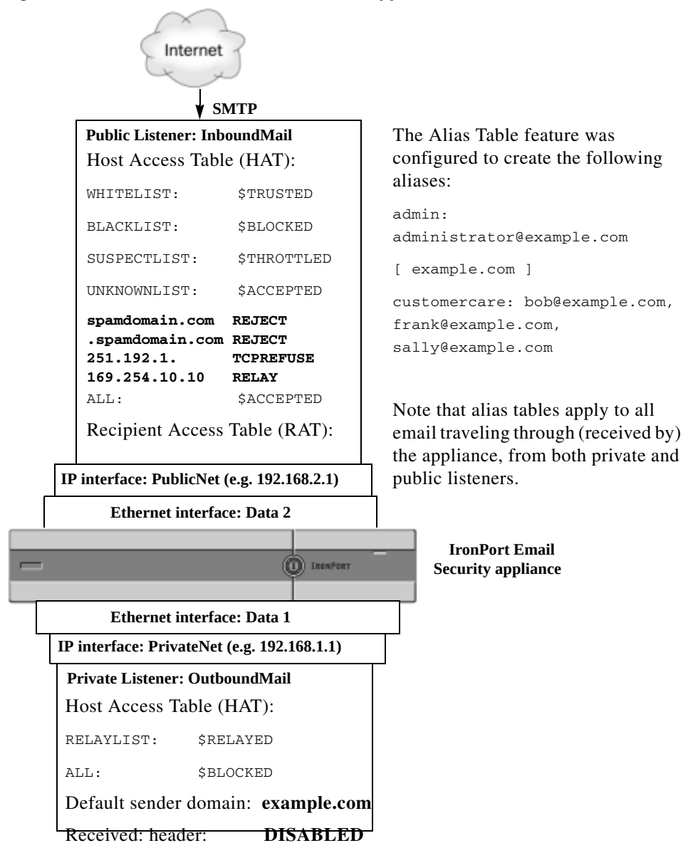
Figure 24-2 Alias Tables Defined for the Appliance
