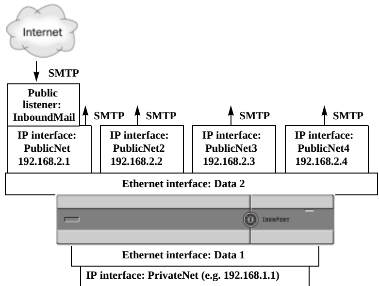
Figure 24-13 Four Virtual Gateway Addresses on One Ethernet Interface
