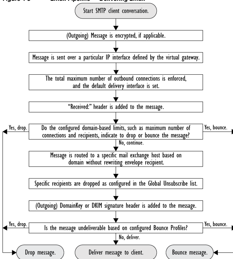
Figure 4-3 Email Pipeline – Delivering Email
