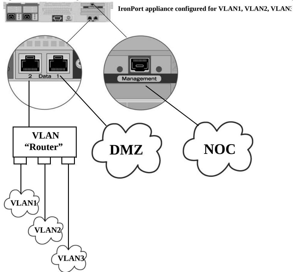
Figure 37-1 Using VLANs to increase the number of networks available on the appliance
