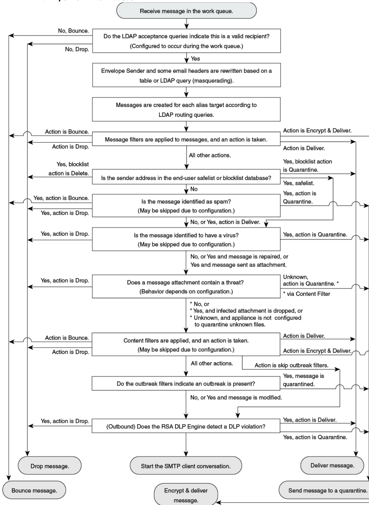
Figure 4-2 Email Pipeline — Work Queue
