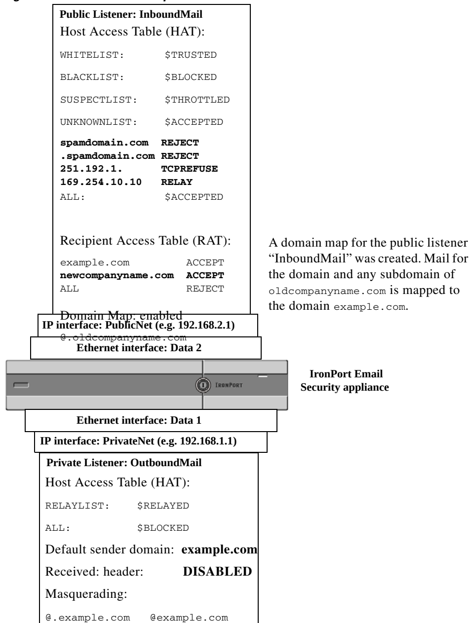
Figure 24-4 Domain Map Defined for a Public Listener
