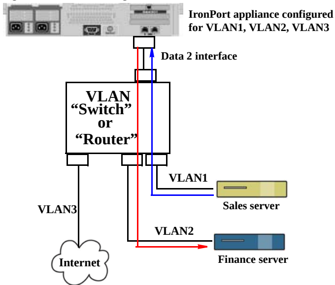
Figure 37-2 Using VLANs to Facilitate Communication Between Appliances
