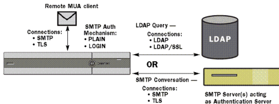
Figure 25-11 SMTP Auth Support: LDAP Directory Store or SMTP Server
