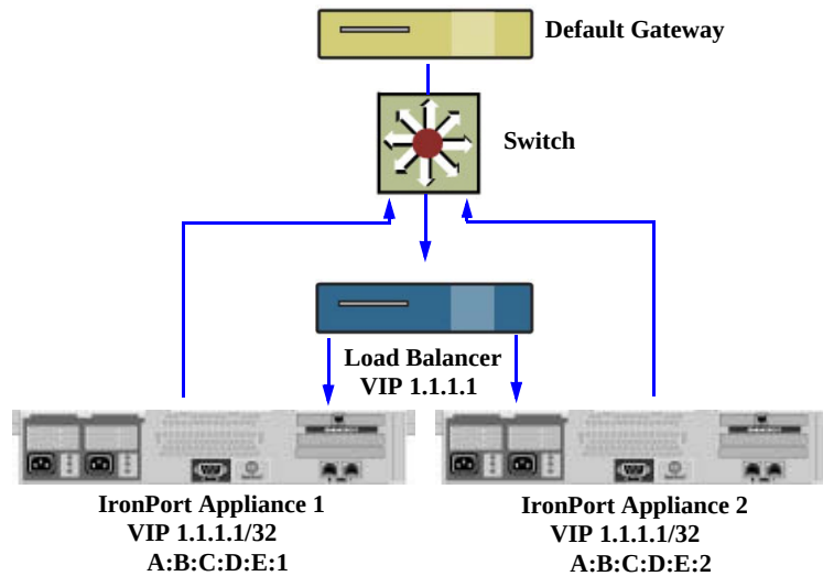
Figure 37-4 Using DSR to Load Balance Between Multiple Email Security Appliances on a Switch
