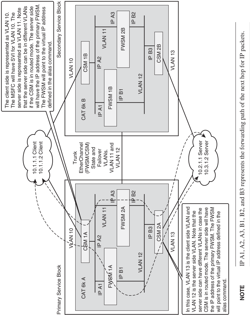
Figure 18-3 High-Level Explanation of Load Balancing Using CSM with Redundancy
