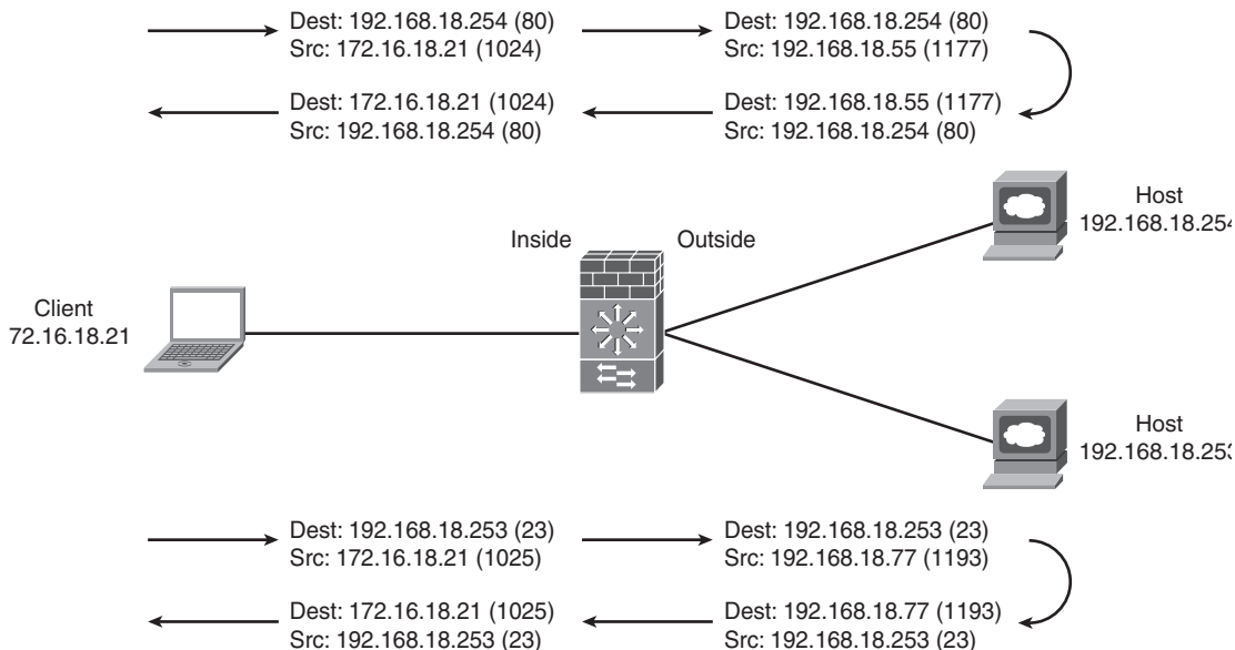
Figure 4-6 Dynamic PAT
