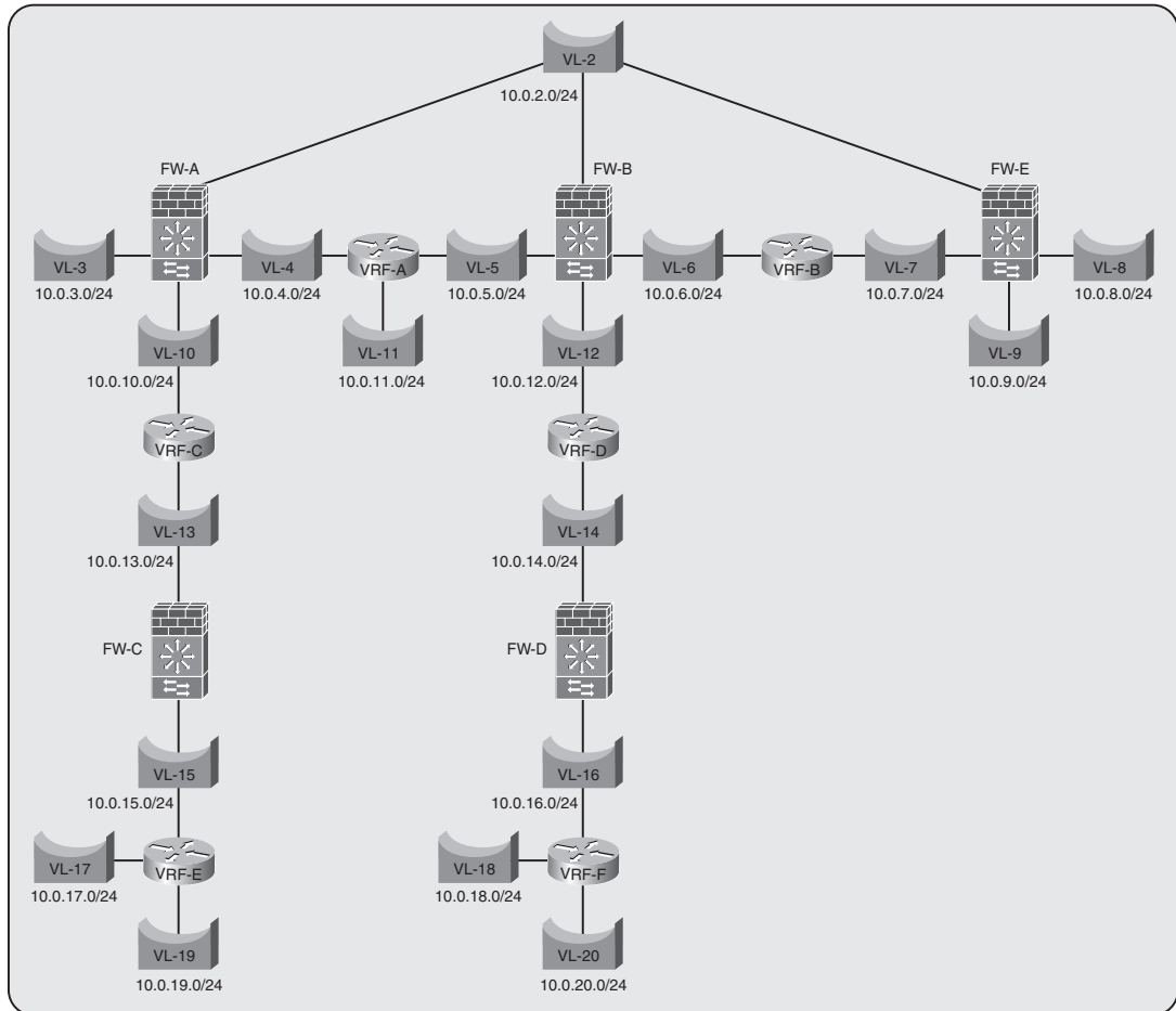
Figure 22-8 Example of Multiple Routing and Firewall Instances
