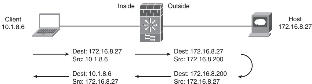
Figure 4-1 NAT
