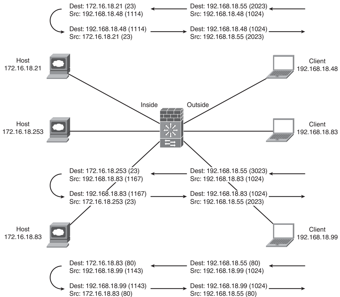
Figure 4-5 Static PAT
