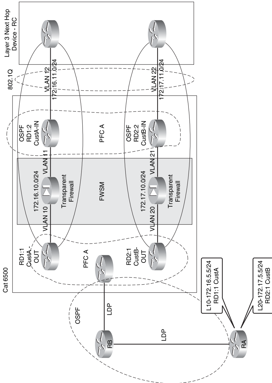
Figure 23-7 Virtualization with FWSM in Layer 2 Mode
