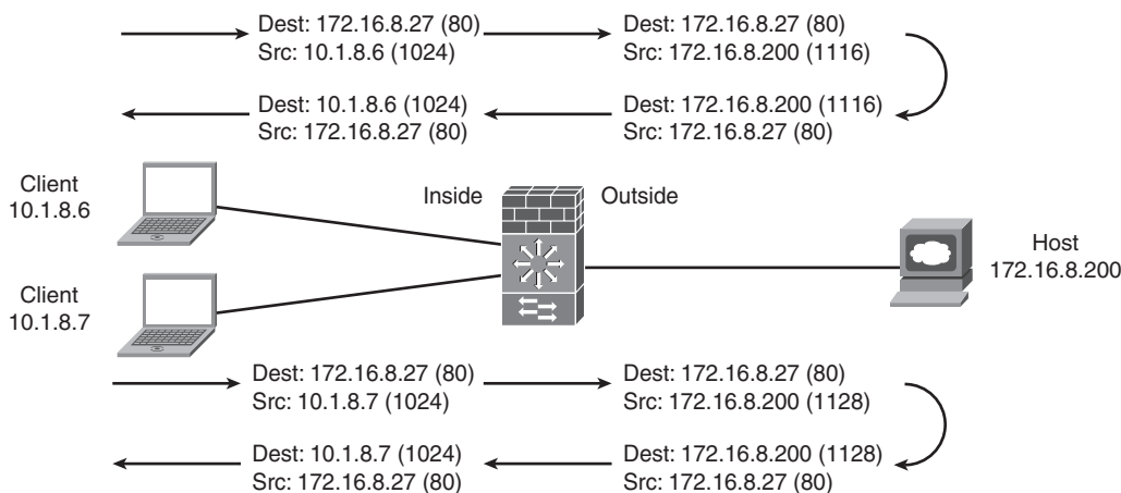
Figure 4-2 PAT Permits Multiple Devices to Share a Single IP Address
