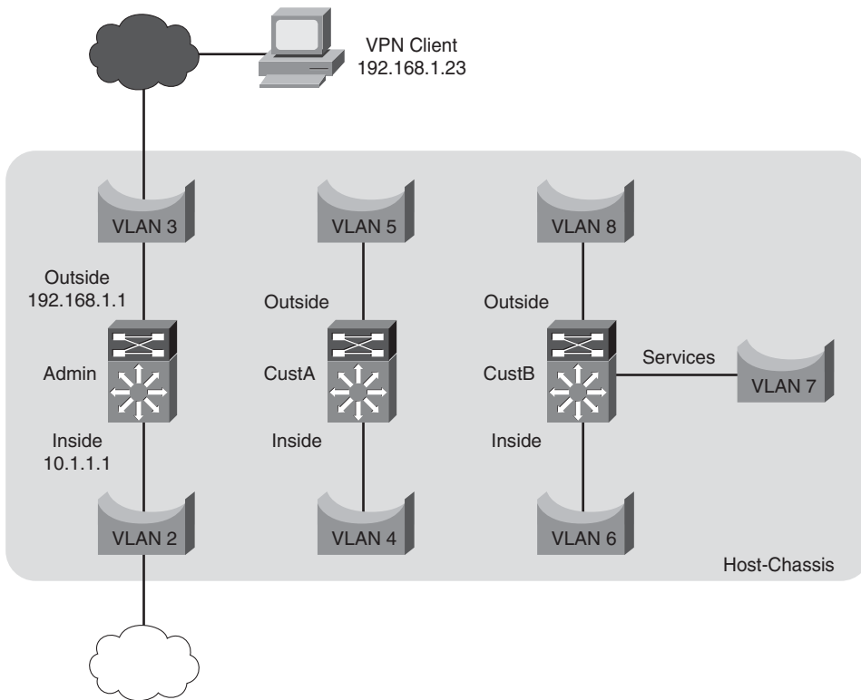
Figure 15-3 Secure Access
