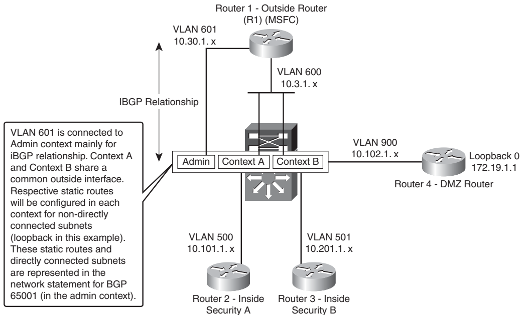
Figure 9-6 BGP Stub Configuration
