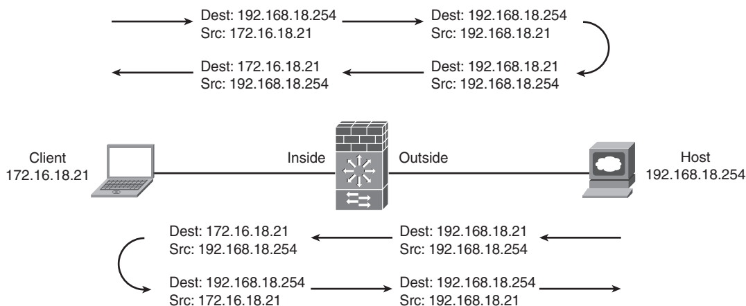
Figure 4-3 Static NAT
