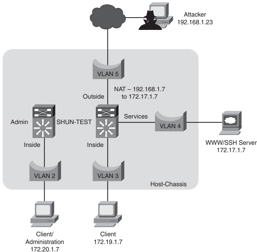
Figure 20-1 Shunning
