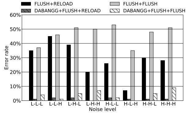
Figure 11: Error rates of different attacks in covert channel scenario at various noise levels.
