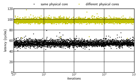
Figure 2: Variation in reload cache hit latency with relative placement of attacker and victim processes. All cores run at the (fixed) base frequency.
