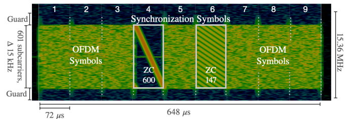
Fig. 5. Spectrum view of a DroneID packet with highlighted Zadoff-Chu synchronization symbols. The signal is the same for the 2.4 GHz and the 5.7 GHz band.
