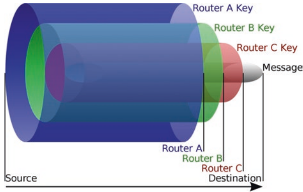
Fig. 1.4 Onion routing technique (Neal 2008)
