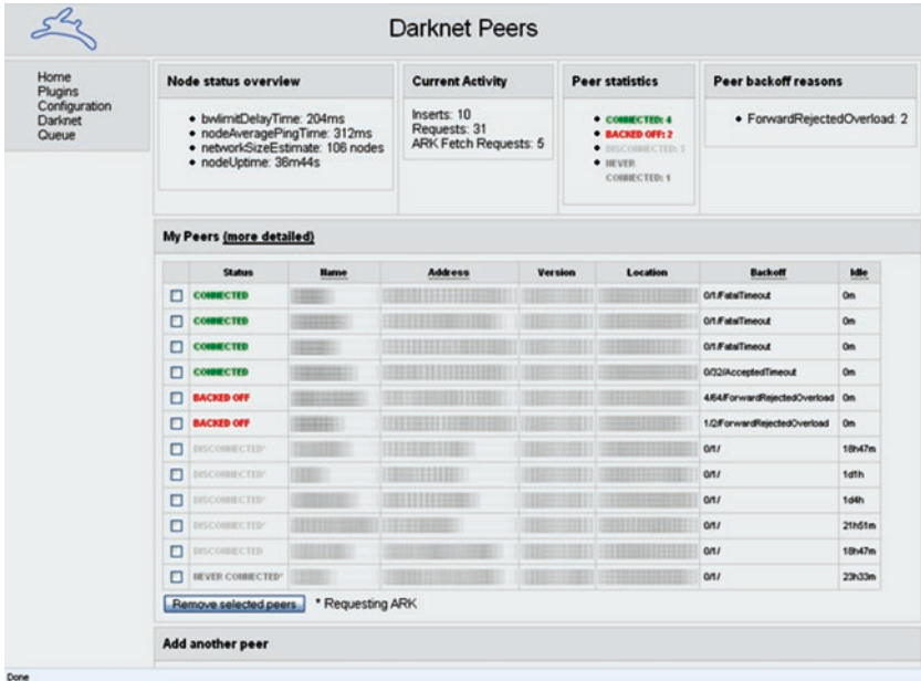
Fig. 1.9 Freenet darknet mode peers (Freenet Project 2018a)
