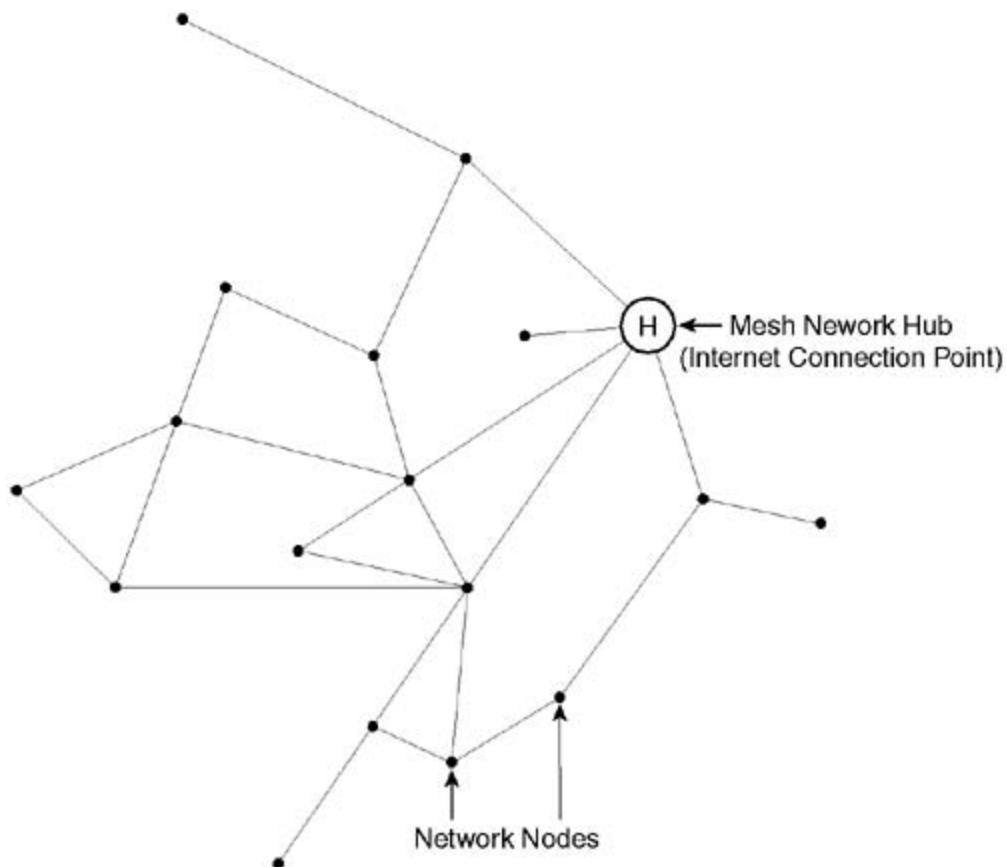
Figure 3-5. Mesh Architecture
