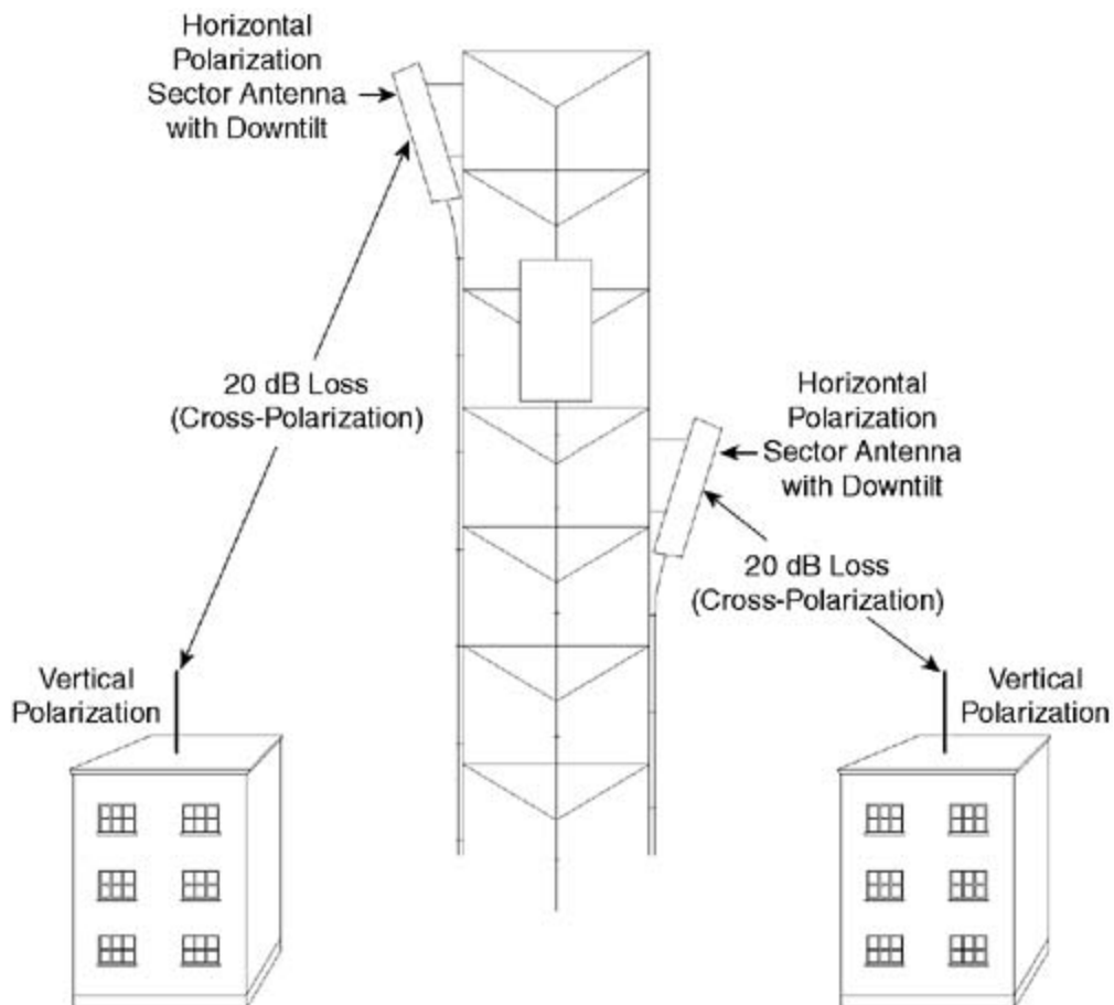
Figure 5-10. Horizontally Polarized Sector Antennas
