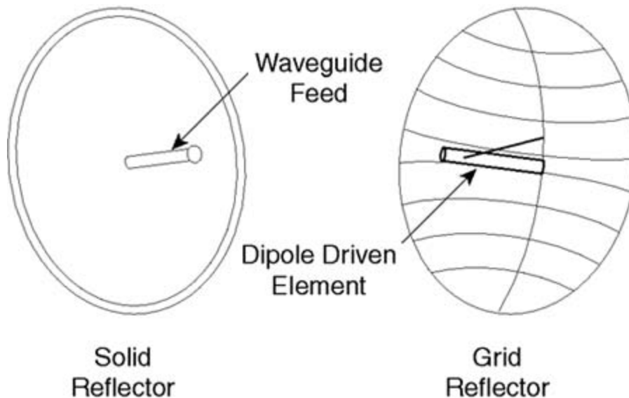
Figure 5-15. Parabolic Antenna
