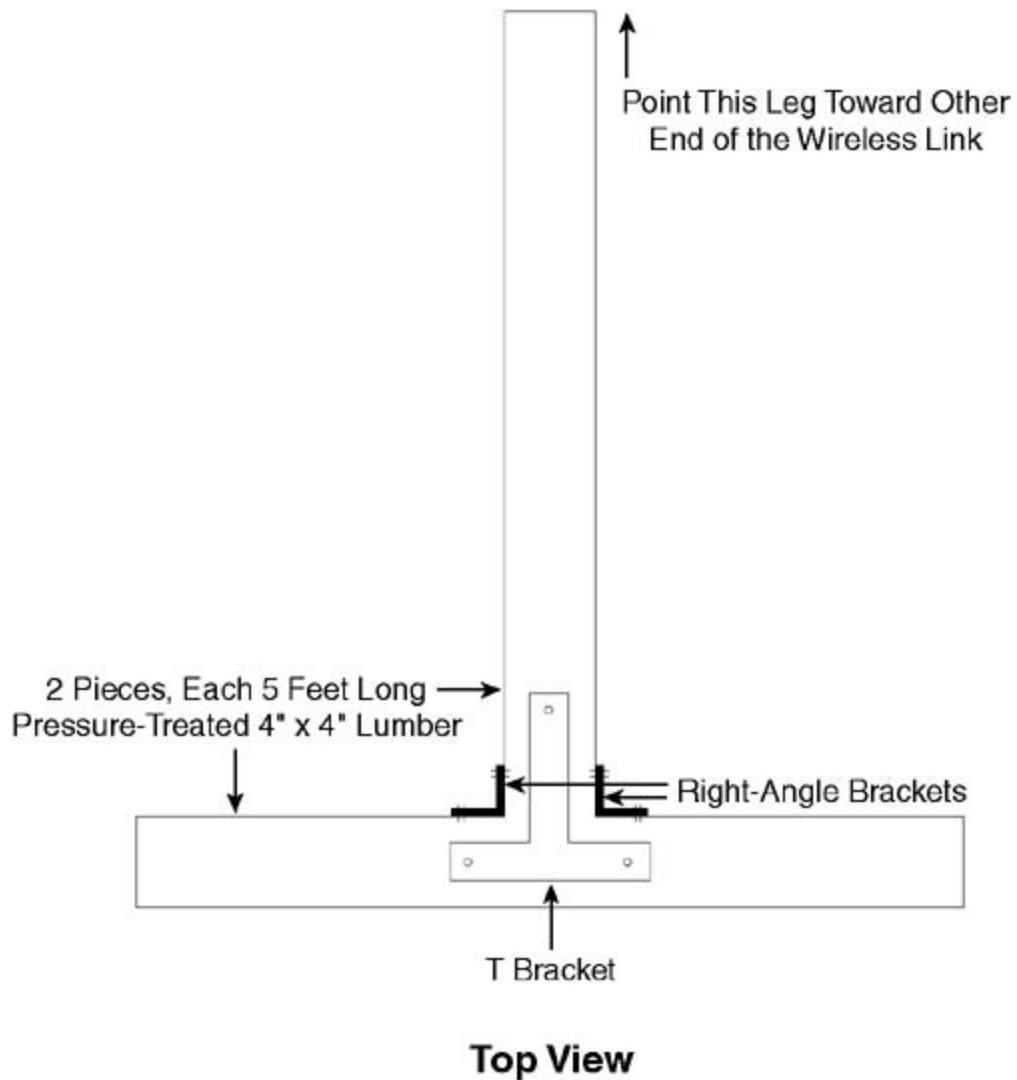
Figure 7-2. Building a Flat-Roof Mast Base
