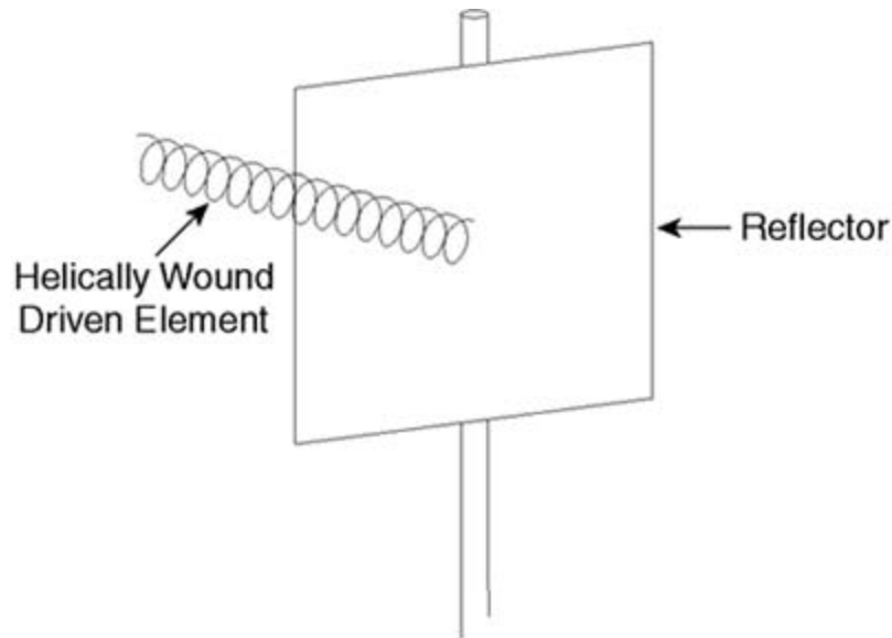
Figure 5-17. Helix Antenna
