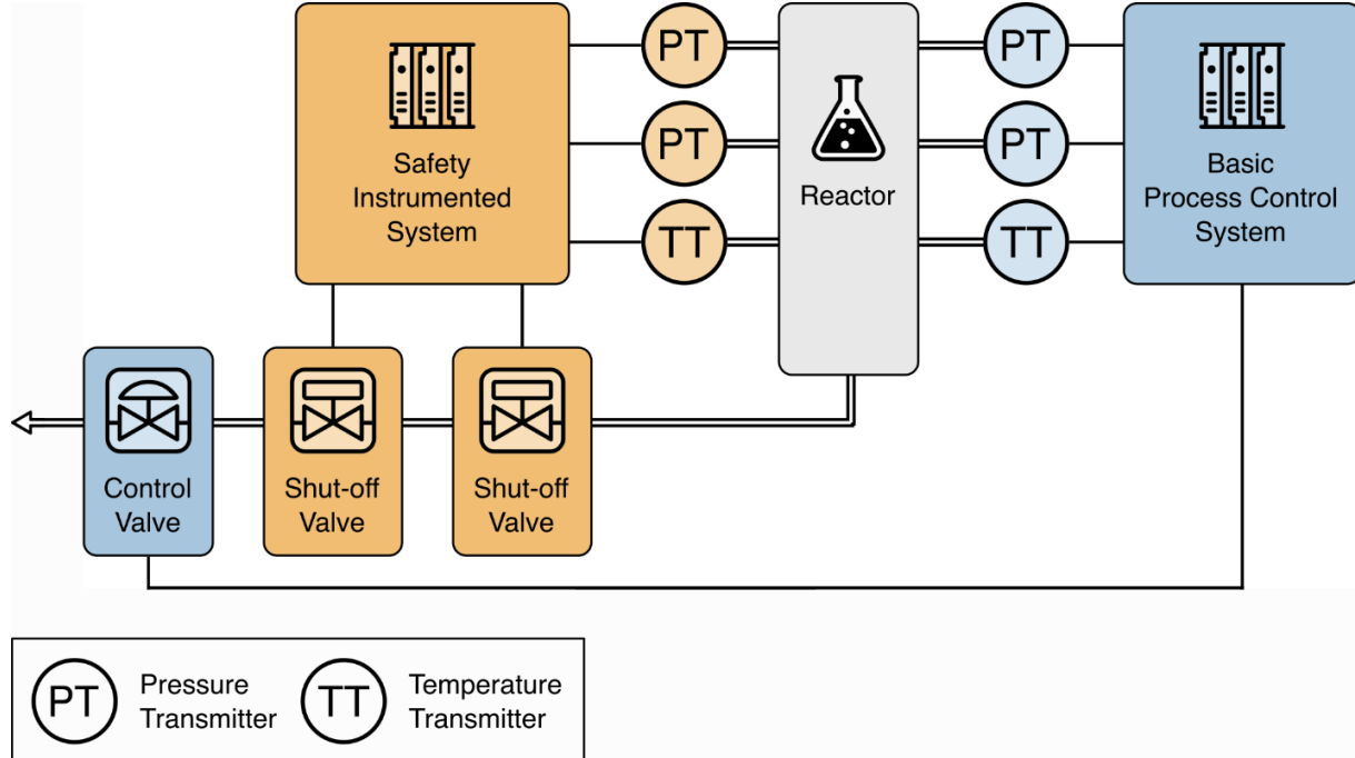
Fig. 11. An SIS implementation example
