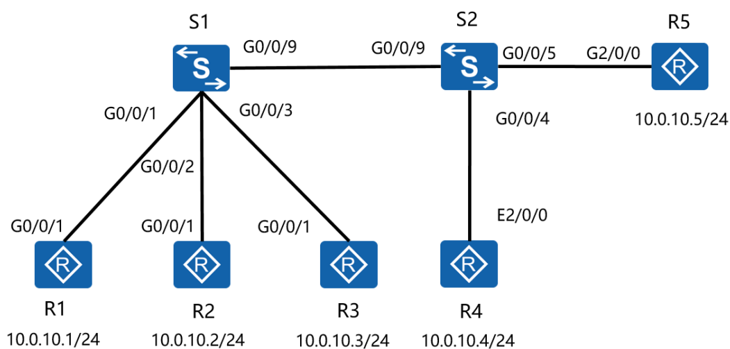
Figure 6-2 MUX VLAN configuration
