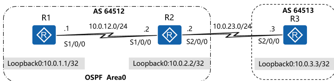
Figure 3-6 BGP troubleshooting
