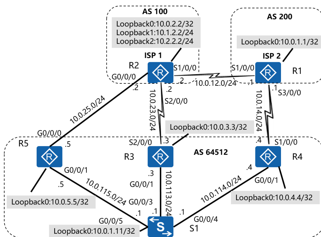
Figure 3-5 BGP multi-homing
