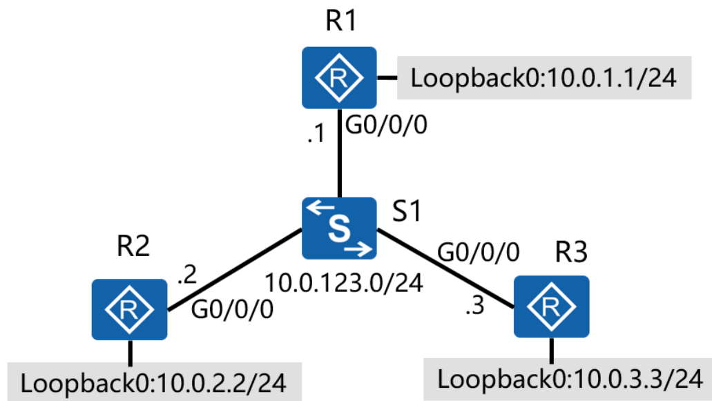
Figure 1-1 Single-area OSPF
