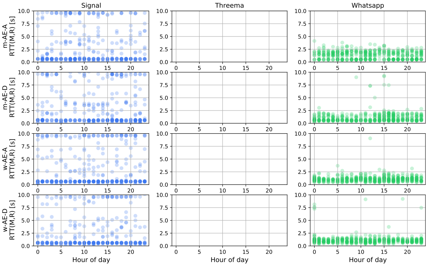
Fig. 21: Distributions of RTT_{M,R} of messages sent to device AE-22 at each location (rows) per hour of day.
