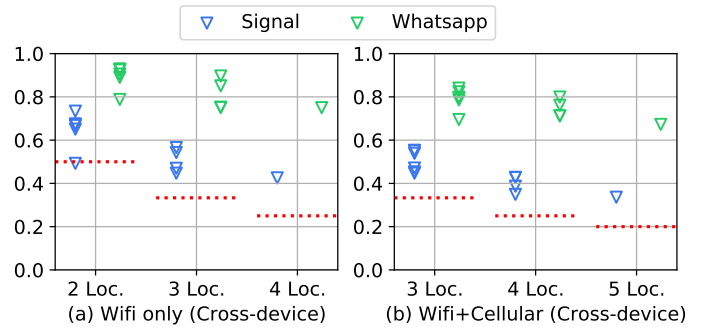
Fig. 11: Overall accuracy of receiver location classification separately for all possible combinations of locations in the UAE. Colors indicate messengers and dotted lines indicate the probability of randomly guessing the correct location.
