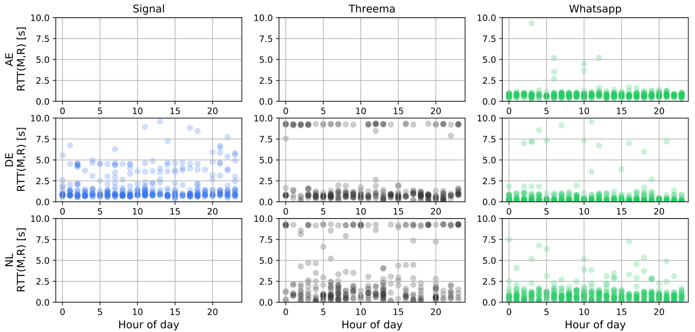
Fig. 17: Distributions of RTT_{M,R} of messages sent from device GR-11 to receivers in different countries per hour of day.
