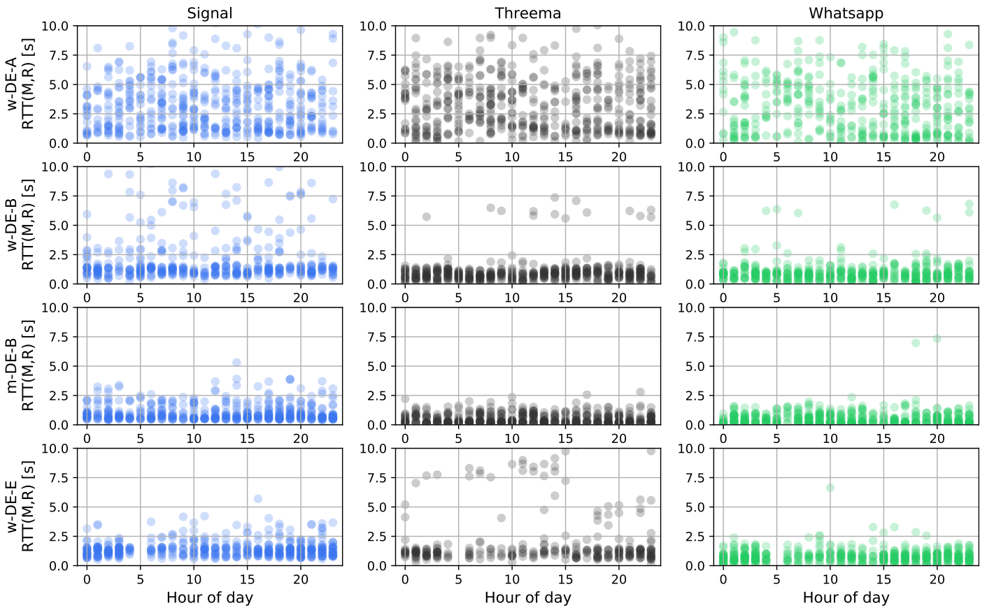
Fig. 20: Distributions of RTT_{M,R} of messages sent to device DE-24 at each location (rows) per hour of day.
