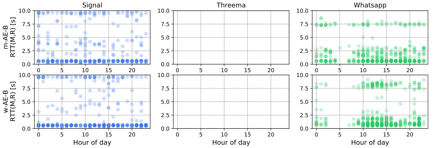
Fig. 22: Distributions of RTT_{M,R} of messages sent to device AE-23 at each location (rows) per hour of day.
