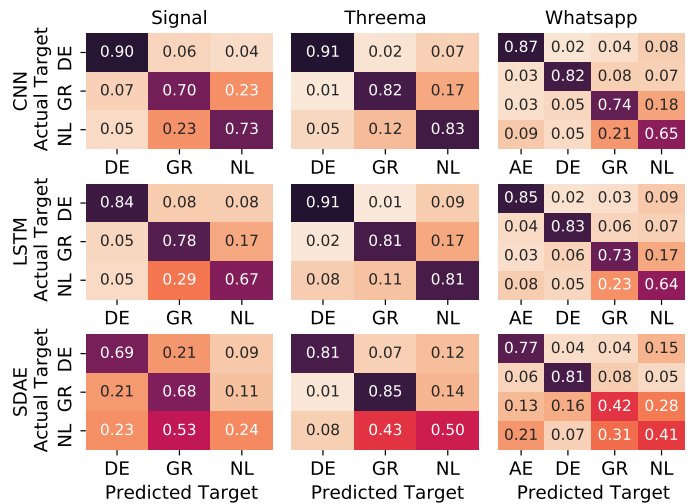
Fig. 7: Detailed classification results for the receiver country based on measurements from sender DE-11 with three different neural network types. For each classification, numbers report precision values, i.e., the fractions of predicted classes (x-axis) given the actual class (y-axis).
