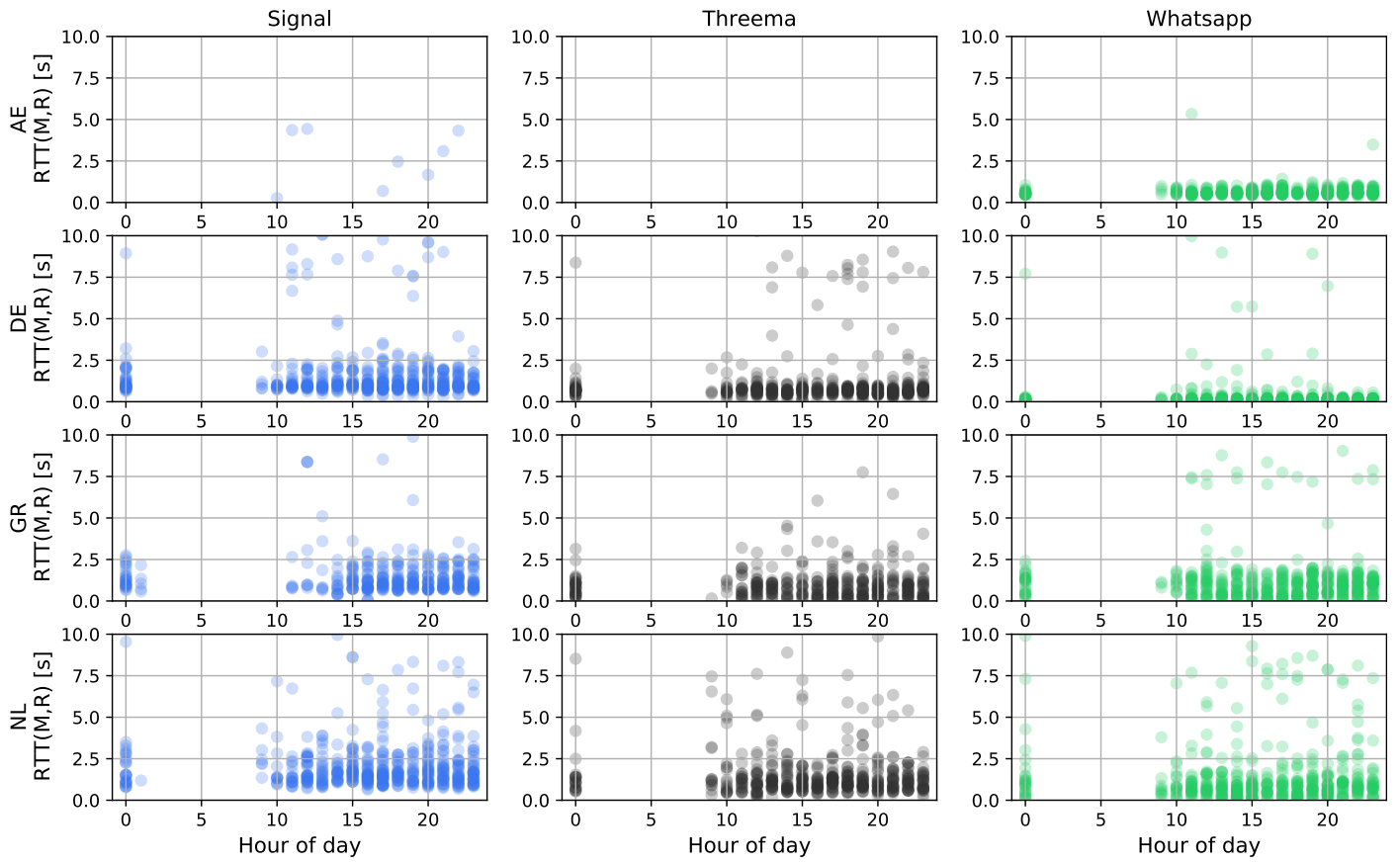
Fig. 16: Distributions of RTT_{M,R} of messages sent from device DE-12 to receivers in different countries per hour of day.
