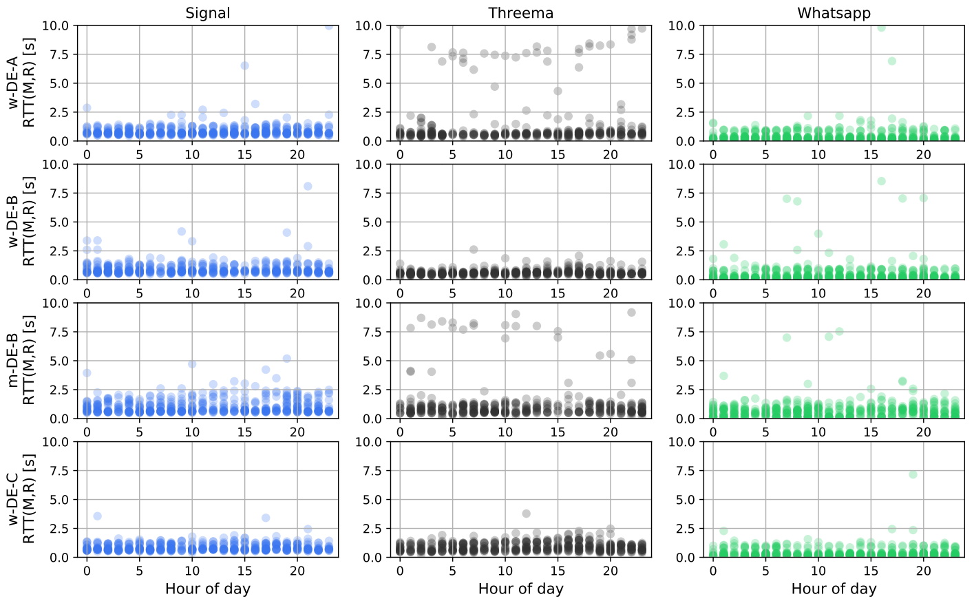
Fig. 18: Distributions of RTT_{M,R} of messages sent to device DE-22 at each location (rows) per hour of day.
