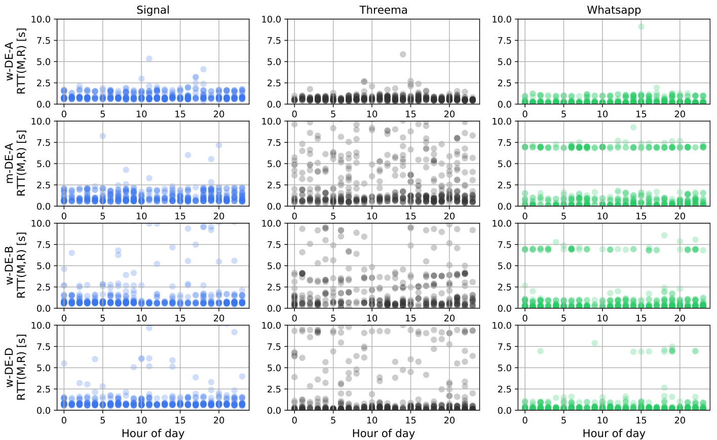
Fig. 19: Distributions of RTT_{M,R} of messages sent to device DE-23 at each location (rows) per hour of day.
