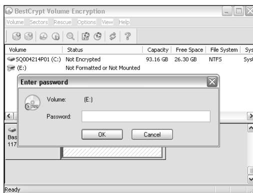
Figure 5.3 A BestCrypt Encrypted Volume
