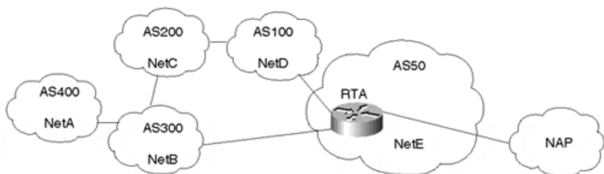
Figure 6-27. Sample Network Topology for Complex Regular Expression
