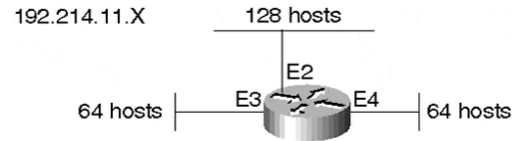
Figure 3-8. Use of VLSM to Split Network Space into Subnets of Unequal Size
