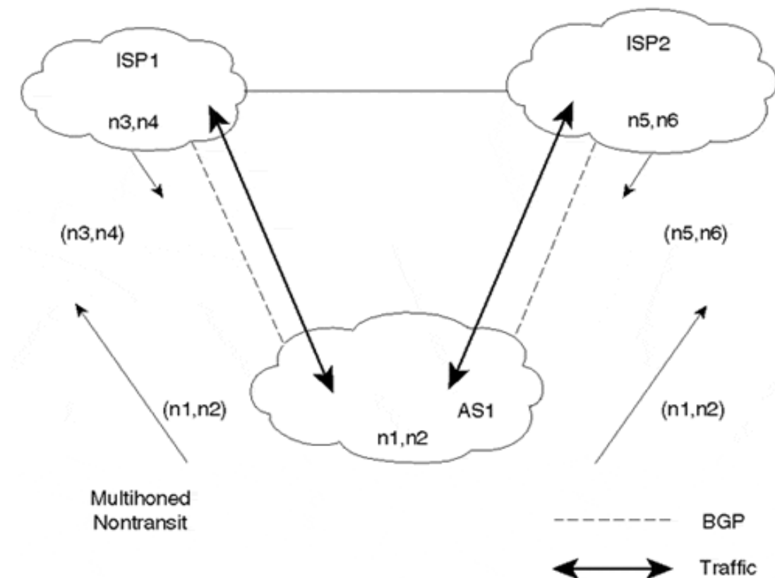
Figure 4-5. Multihomed Nontransit AS Example
