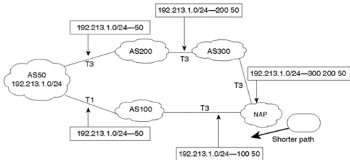
Figure 6-22. Routing Environment Before Dummy AS Is Prepended
