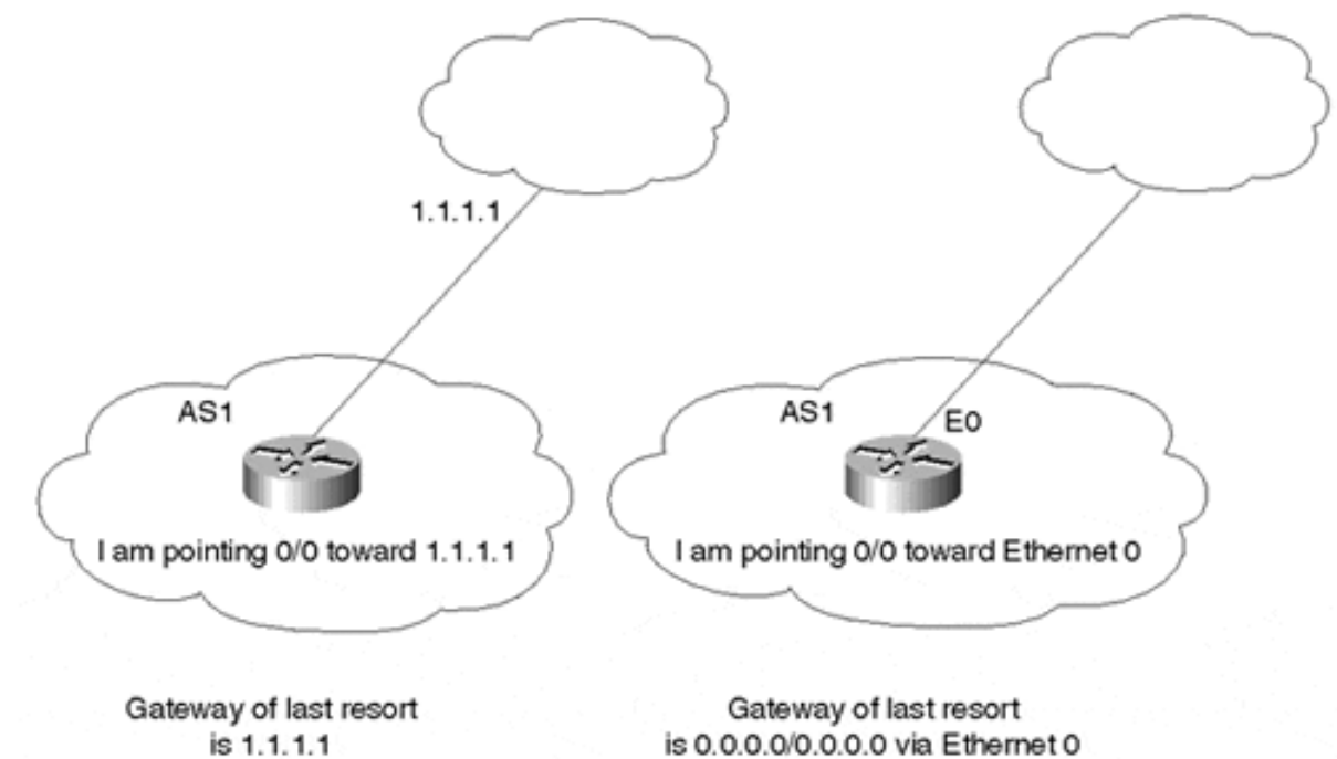
Figure 7-3. Statically Set Defaults
