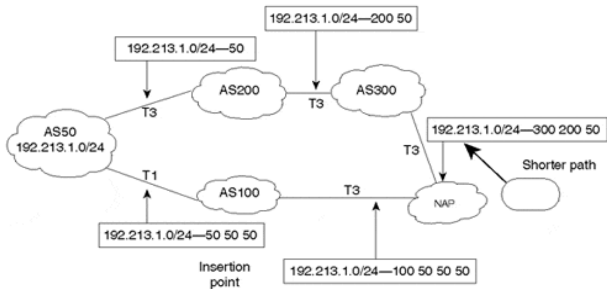
Figure 6-23. Routing Environment After Dummy AS Is Prepend
