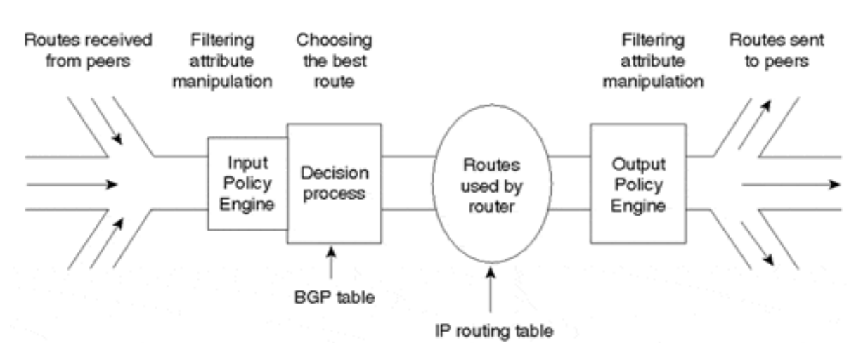
Figure 6-8. Routing Process Overview
