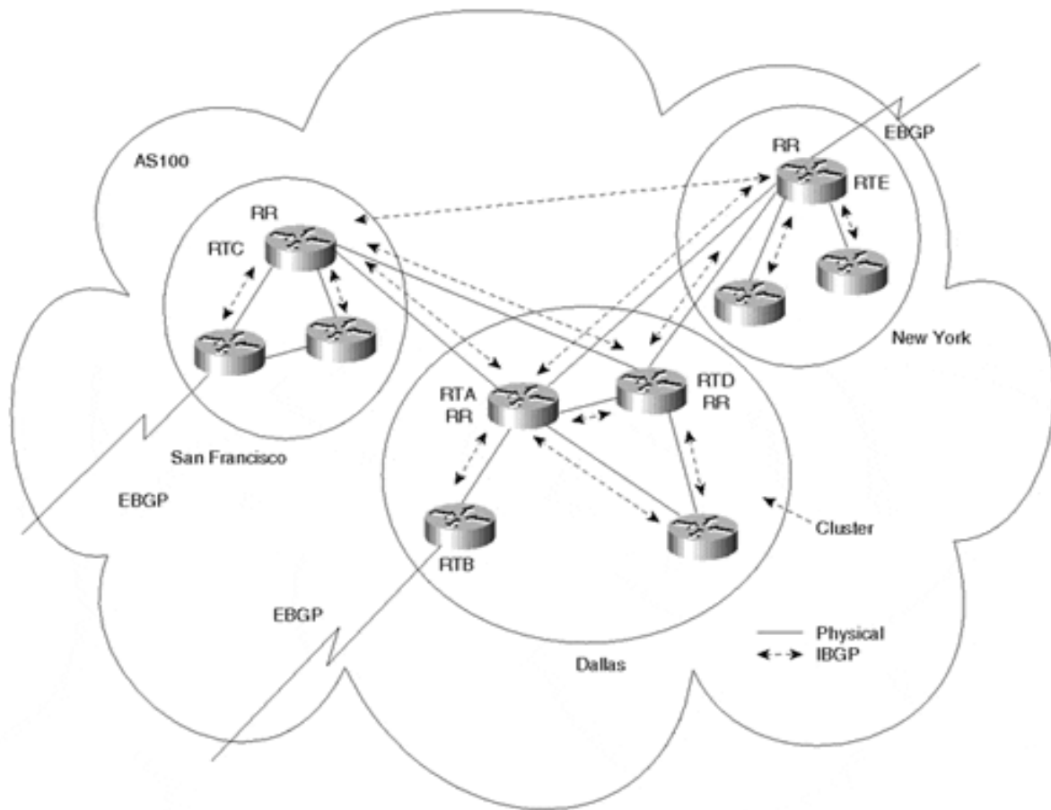
Figure 9-5. Complex Multiple Route Reflector Environment
