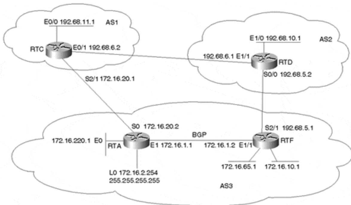
Figure 11-6. Applying BGP Attributes
