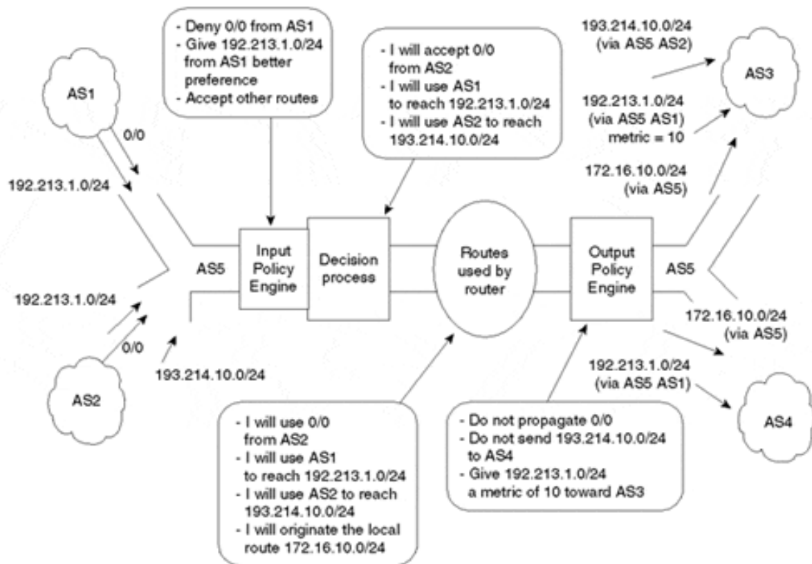
Figure 6-10. Sample Routing Environment
