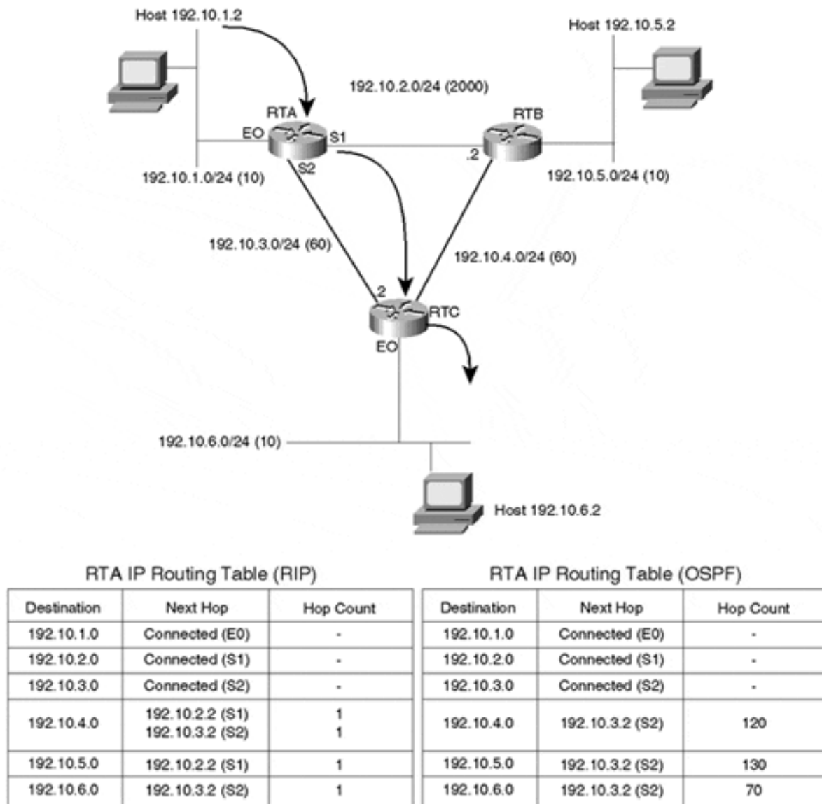
Figure 4-1. Basic Routing Behavior
