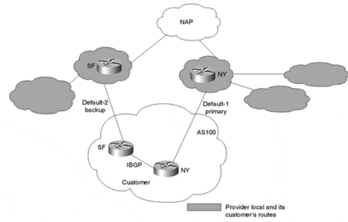
Figure 7-15. Multihoming to Two Providers Plus Partial Routing
