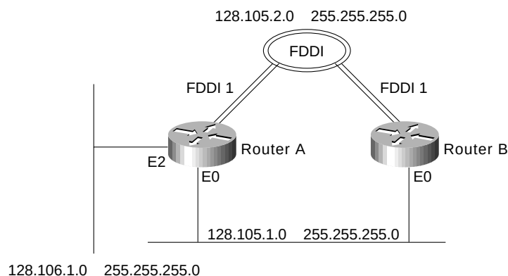
Figure 4-4 Route summarization.
