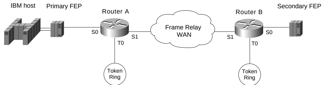
Figure 7-6 Topology for basic STUN: example 2.
