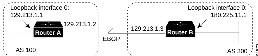
Figure 12-4 EBGp Multihop
