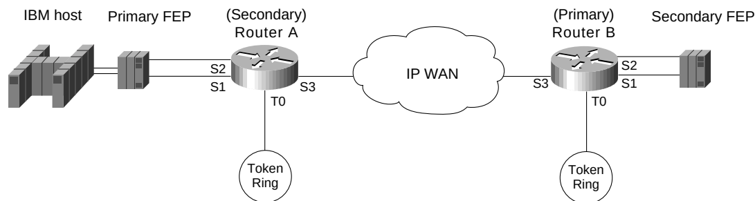
Figure 7-8 The SDLC-TG STUN topology.
