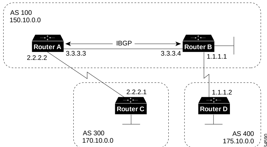
Figure 12-7 Disabled Synchronization
