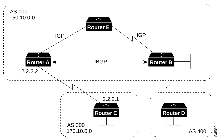
Figure 12-6 Synchronization
