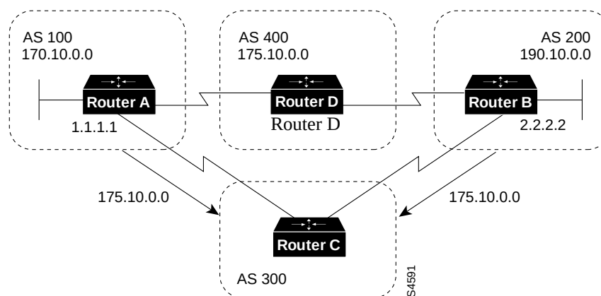
Figure 12-16 Weight Example
