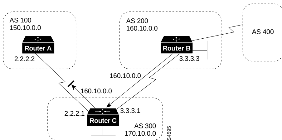
Figure 12-21 AS_path Filtering
