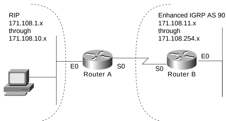
Figure 4-5 Redistributing RIP routes into Enhanced IGRP.
