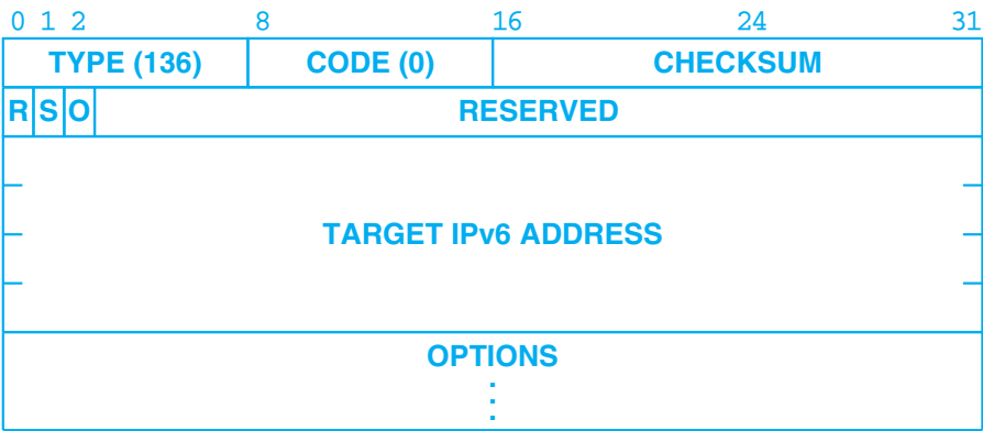
Figure 22.9 The format of an ICMPv6 Neighbor Advertisement message.
