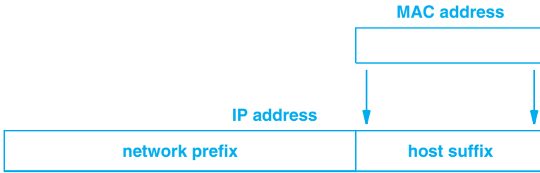
Figure 6.1 An illustration of a direct mapping scheme in which a computer's hardware address is embedded in the computer's IP address.
