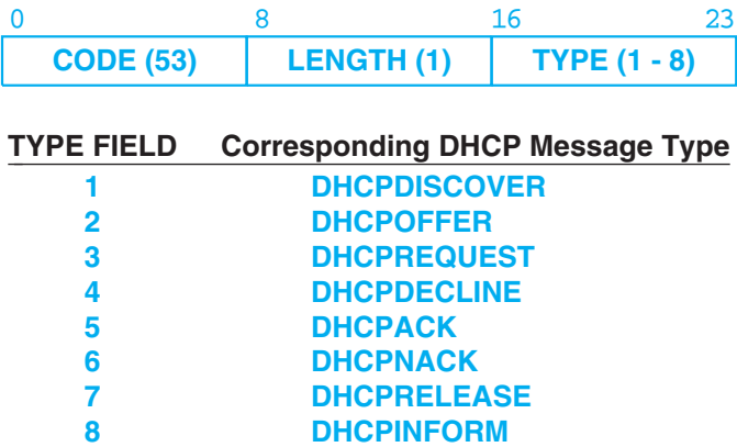
Figure 22.4 The format of a DHCP option used to specify the DHCP message type with a list of the possible values for the third octet.
