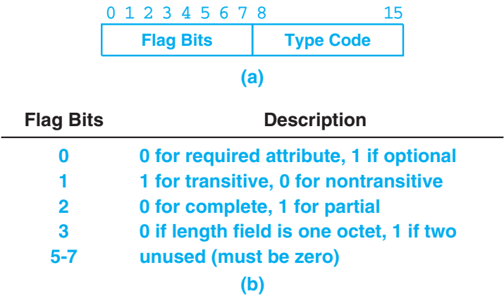
Figure 13.8 (a) The two-octet type field that appears before each BGP attribute path item, and (b) the meaning of each flag bit.
