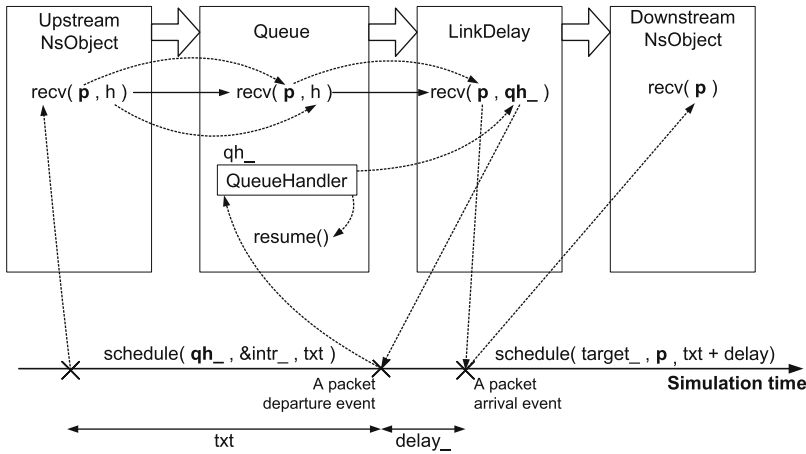
Fig. 7.3. Diagram of callback mechanism for a queue unblocking process.
