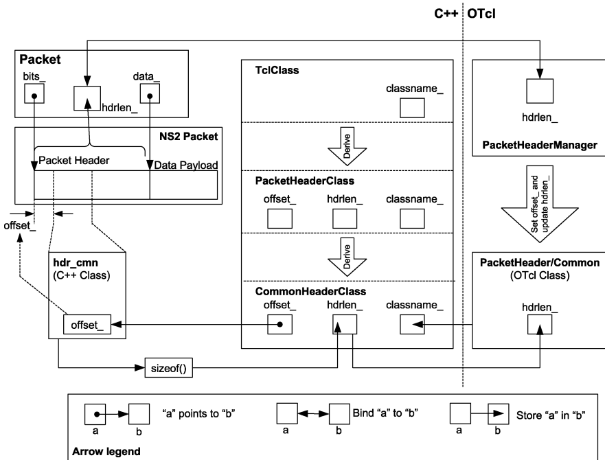
Fig. 8.9. A schematic diagram of a static mapping object class_cmnhdr , class_hdr_cmnh , class PacketHeader/Common , and class Packet .
