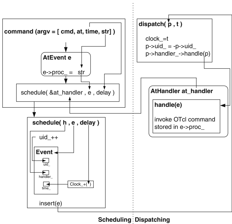
Fig. 4.3. Scheduling and dispatching mechanism of an AtEvent .
