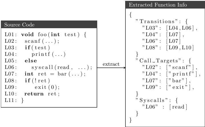
Figure 11.2: A simplified example of the information that is extracted from a function. Transitions identifies control-flow transfers between basic blocks, Call Targets the location of a call to another function and the targets name, Syscalls the location of the syscall and the corresponding syscall number.
