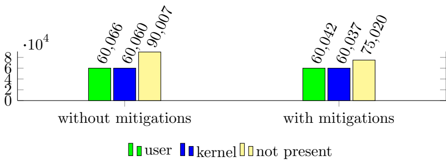
Figure 6.2: Issued load \mu OPs for user and kernel addresses (Intel). Only invalid loads from non-present pages are reissued.
