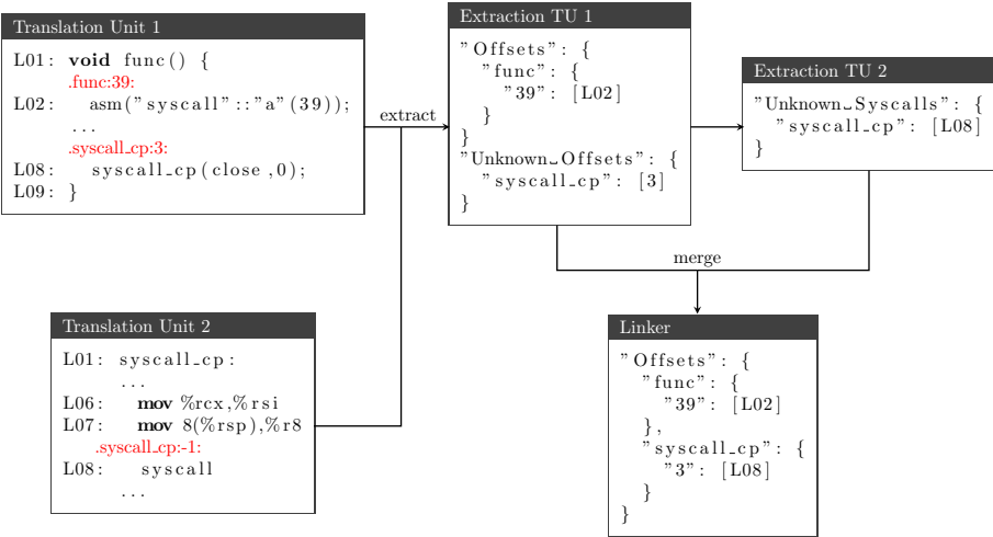
Figure 11.3: A simplified example of the syscall-origin extraction. Inserted red labels mark the location of a syscall and encode available information. The extraction deconstructs the label and calculates the offset using the label’s address from the symbol table. The linker combines the information from each translation unit and generates the final syscall-origin mapping.
