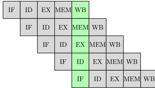
Figure 2.5: An example of a simple 5-stage pipeline. The stages are Instruction Fetch (IF), Instruction Decode (ID), Execute (EX), Memory Access (MEM), and Write Back (WB).
