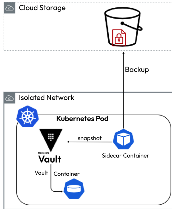
Figure 6.1 – Hashicorp Vault sidecar for backup
