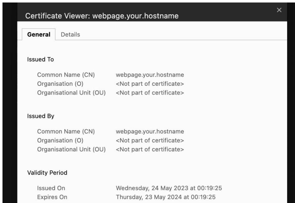
Figure 2.1 – SSL certificate
