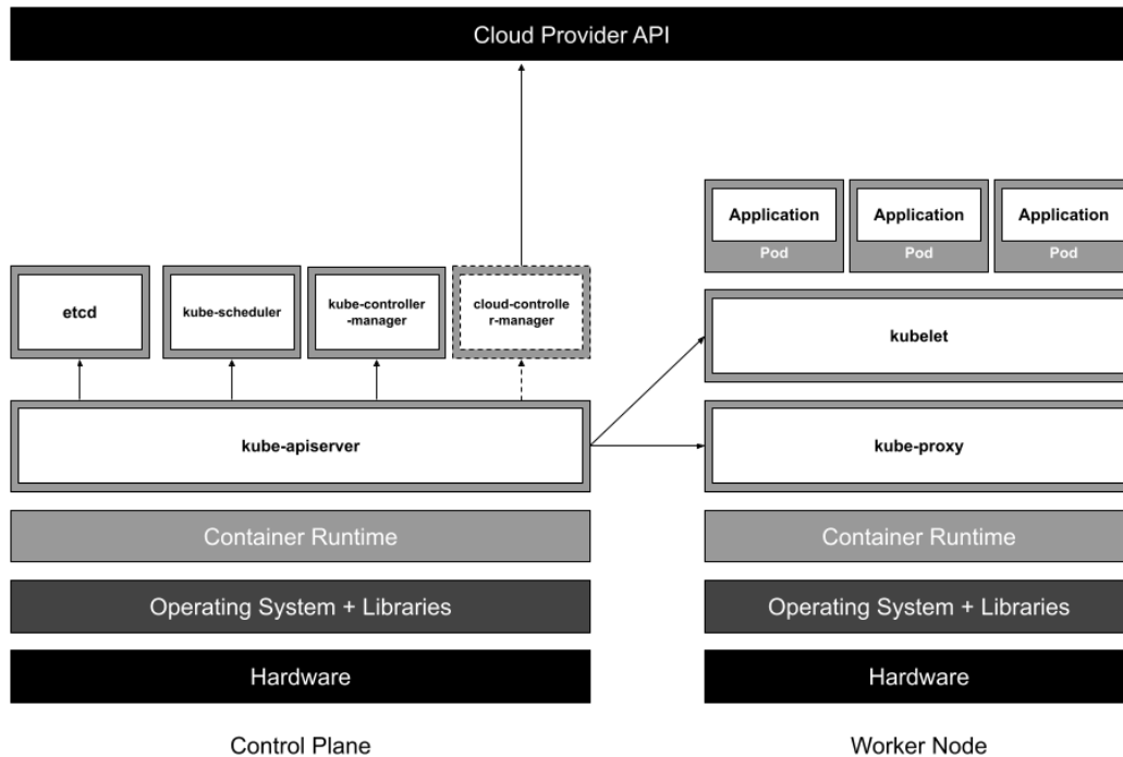
Figure 1.2 – Kubernetes components
