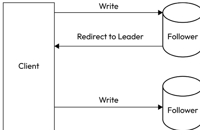
Figure 11.4 – Client redirect
