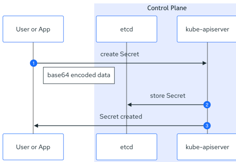
Figure 1.4 – Secret creation
