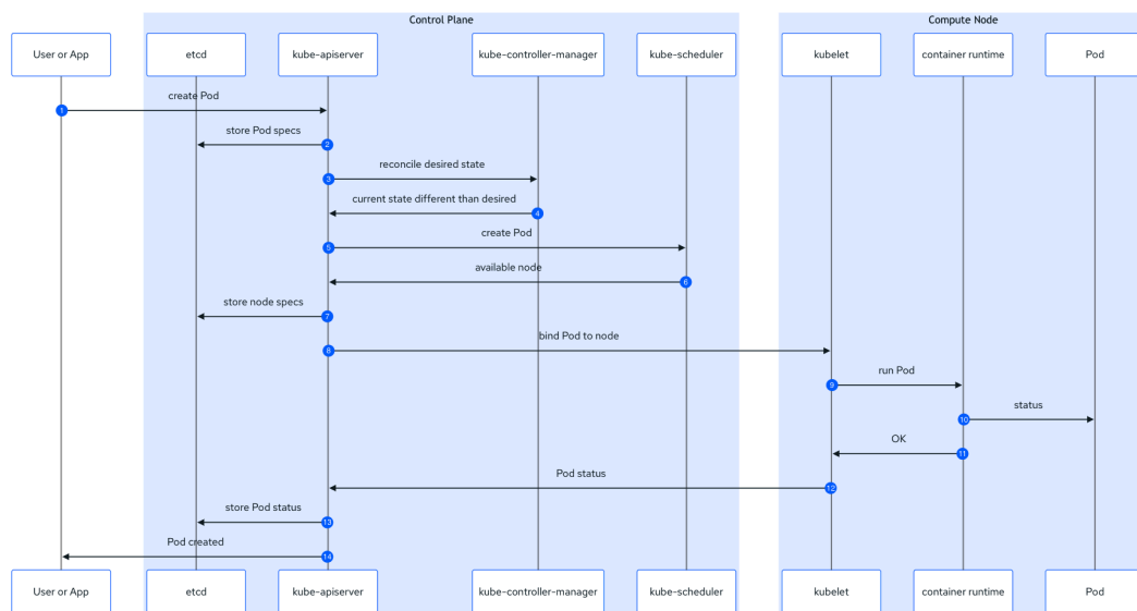
Figure 1.3 – Kubernetes Pod creation
