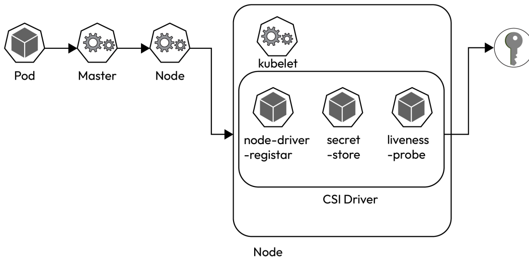
Figure 9.1 – Azure Key Vault integration
