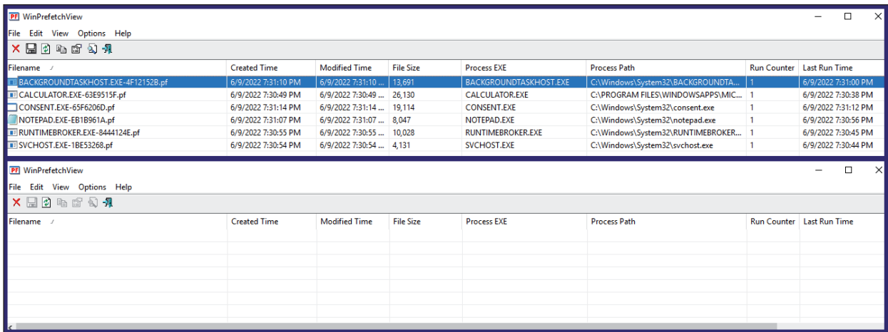
Figure 20: Prefetch files before and after manually exceeding the limit for allowed traces in Nirsoft’s WinPrefetchView.
