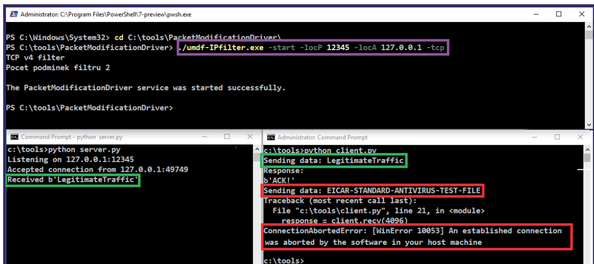
Figure 15: The EICAR test string triggered the blocking of server-client connection (lower pane) after the WFP callout is created on the local TCP connection over port 12345 (upper pane).
