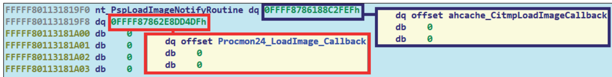
Figure 11: PspLoadImageNotifyRoutine function table with two callbacks for an allowlisted ahcache.sys and targeted Procmon24.sys .
