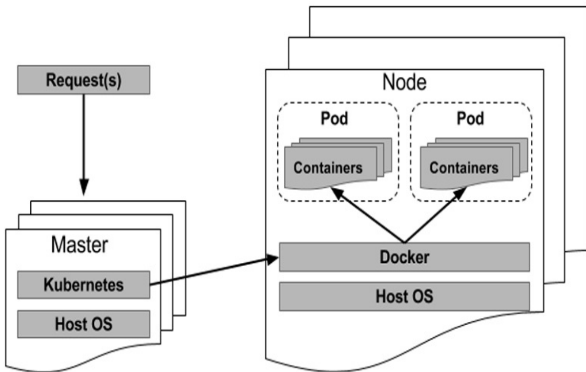
Figure 2. A General Model of Pod Creation/Management
