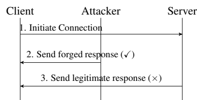
Figure 1: Sequence Diagram of Man-on-the-Side (MotS) attack.
