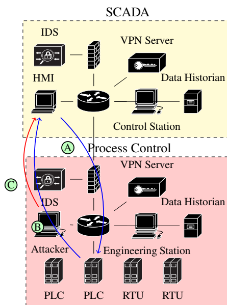
Figure 3: A generalised network diagram showing two enclaves: SCADA and Process Control.
