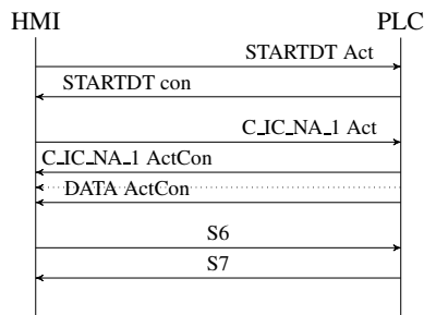
Figure 4: Sequence diagram of a Human Machine Interface (HMI) performing an General Interrogation (GI) command on a Programmable Logic Controller (PLC). The dotted line shows the injected response.
