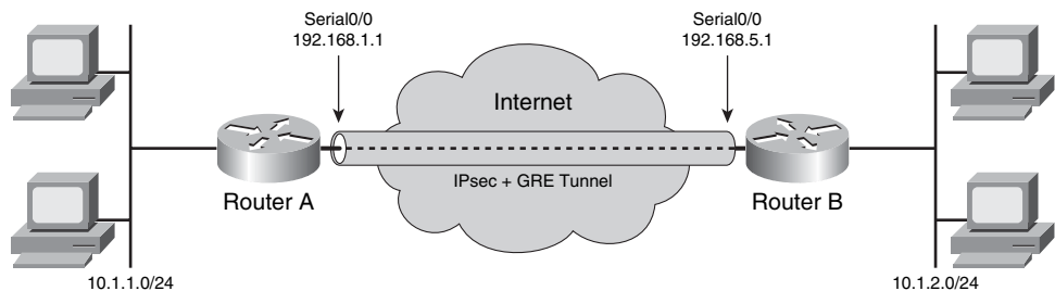
Figure 7-6 IPsec + GRE VPN Deployment Using ESP Tunnel Mode
