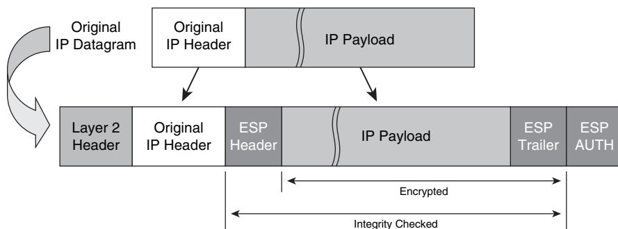
(a) IP Datagram – ESP Transport Mode
