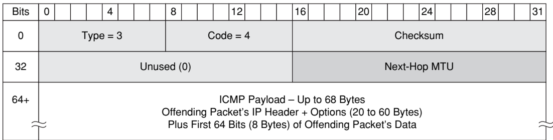
Figure B-7 ICMP Header—Destination Unreachable, Fragmentation Needed and Don't Fragment was Set Error Message
