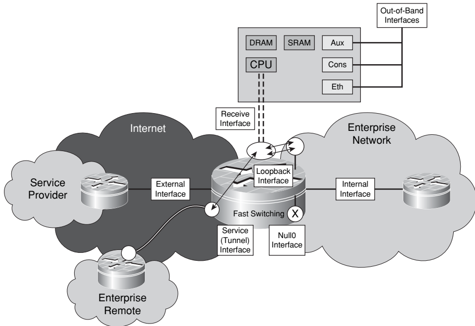
Figure 3-2 External, Internal, Out-of-Band, Loopback, Null0, Service, and Receive Interfaces
