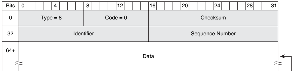
Figure B-5 ICMP Header—Echo Request/Echo Reply Query Message
