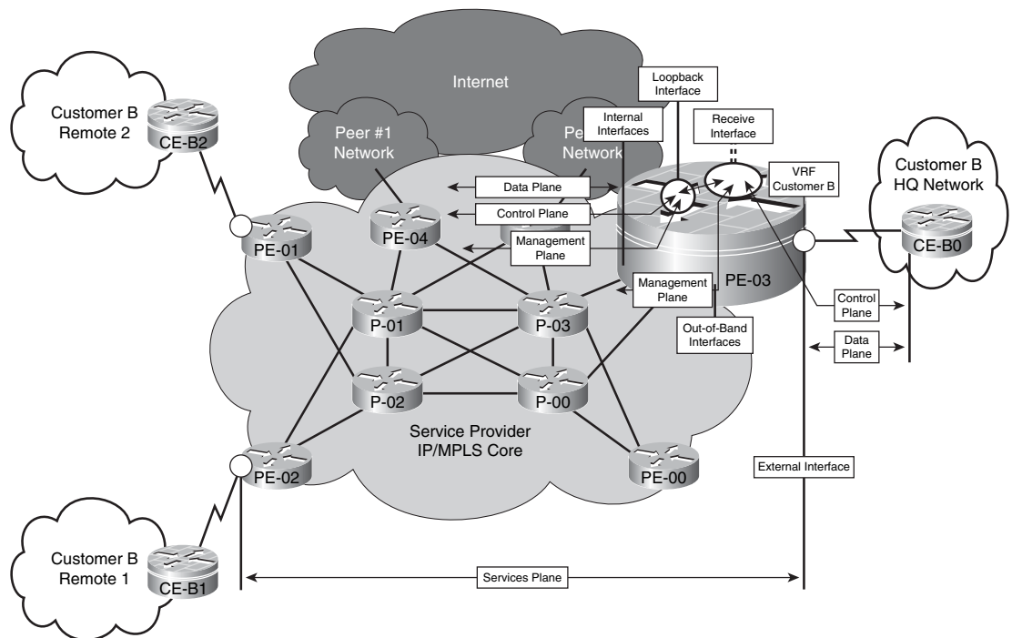
Figure 9-5 IP Traffic Plane Relationships to Router Interfaces for MPLS VPN Case Study 2
