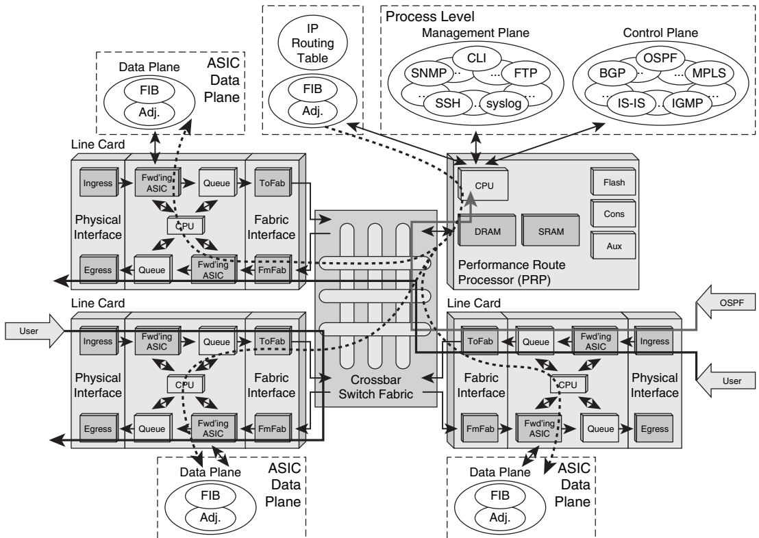
Figure 1-17 Distributed ASIC-Based Router Architecture
