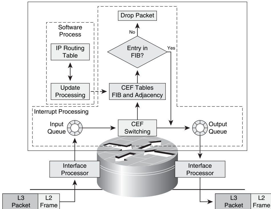
Figure 1-13 Illustration of CEF Switching
