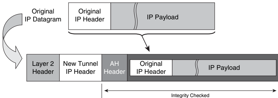
(b) IP Datagram – AH Tunnel Mode
