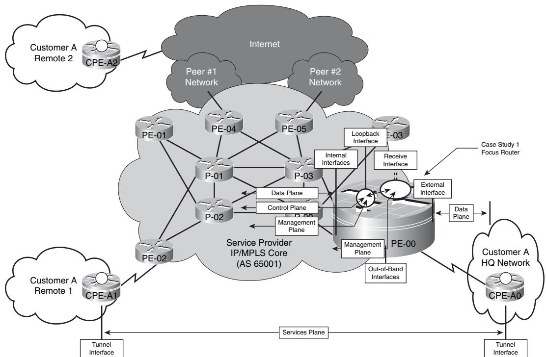
Figure 9-3 IP Traffic Plane Relationships to Router Interfaces for Internet-Based IPsec VPN Case Study 1
