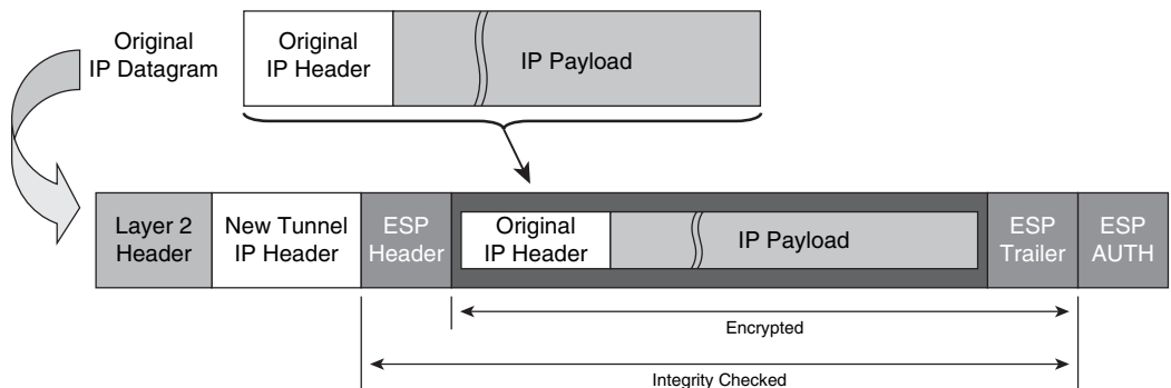
(b) IP Datagram – ESP Tunnel Mode
