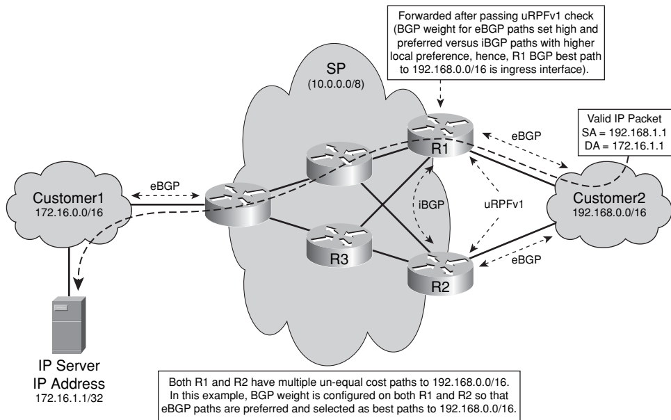
Figure 4-5 Strict uRPF Example Using Cisco IOS BGP Weight Attribute Within Multihomed Topologies
