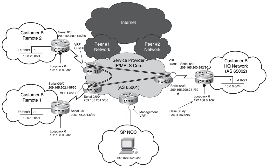
Figure 8-4 Conceptual Enterprise Network Architecture for MPLS VPN Connectivity Case Study 2
