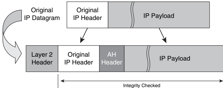
(a) IP Datagram – AH Transport Mode
