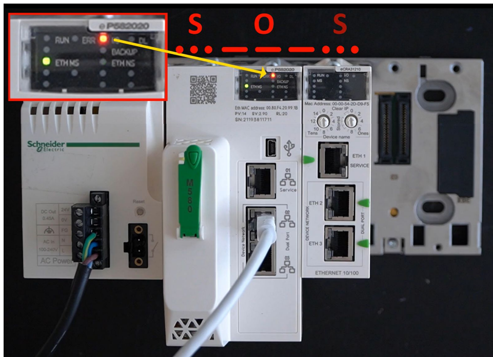
Screenshot from a demo video, showing the developed exploit blinking an LED on the Modicon PLC, sending out the S-O-S morse code.
