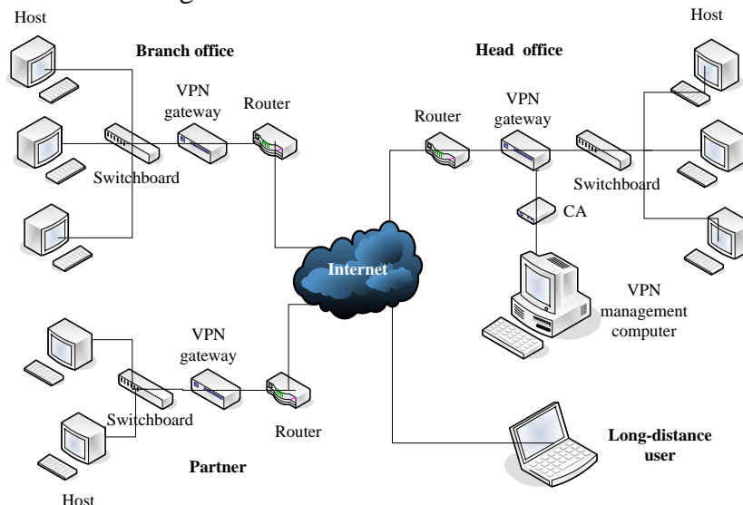
Figure 2. VPN construction
