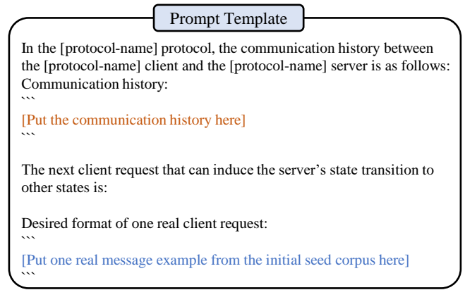
Fig. 9. The prompt template for obtaining the next client request that can induce the server’s state transition to other states.
