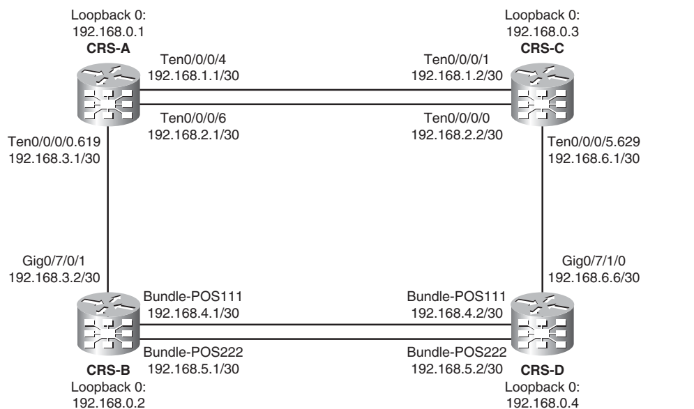
Figure 9-2 MPLS Network
