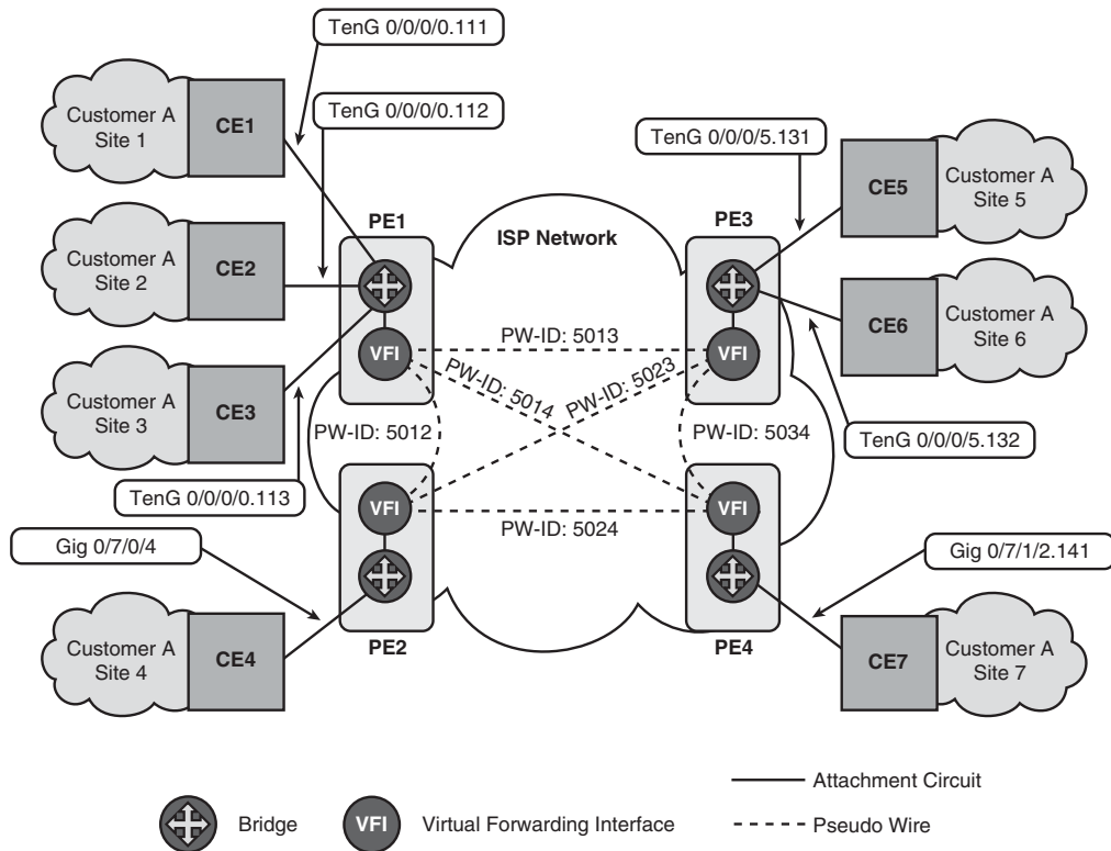
Figure 9-9 VPLS Service Scenario
