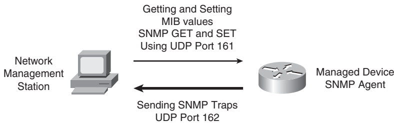
Figure 5-1 SNMP Traffic
