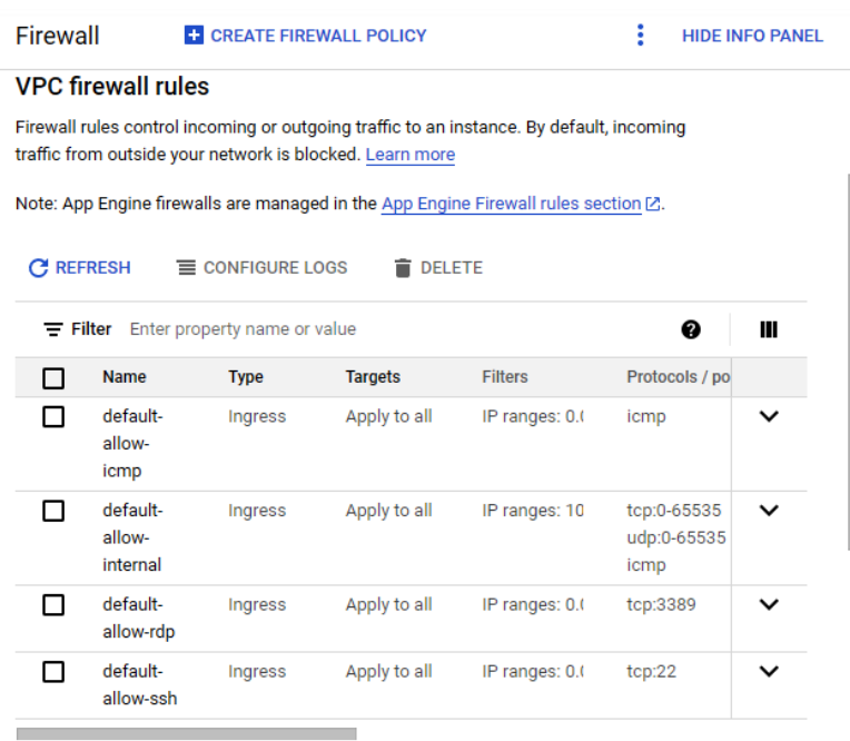
Figure 4.35 – GCP – VPC firewall rules
