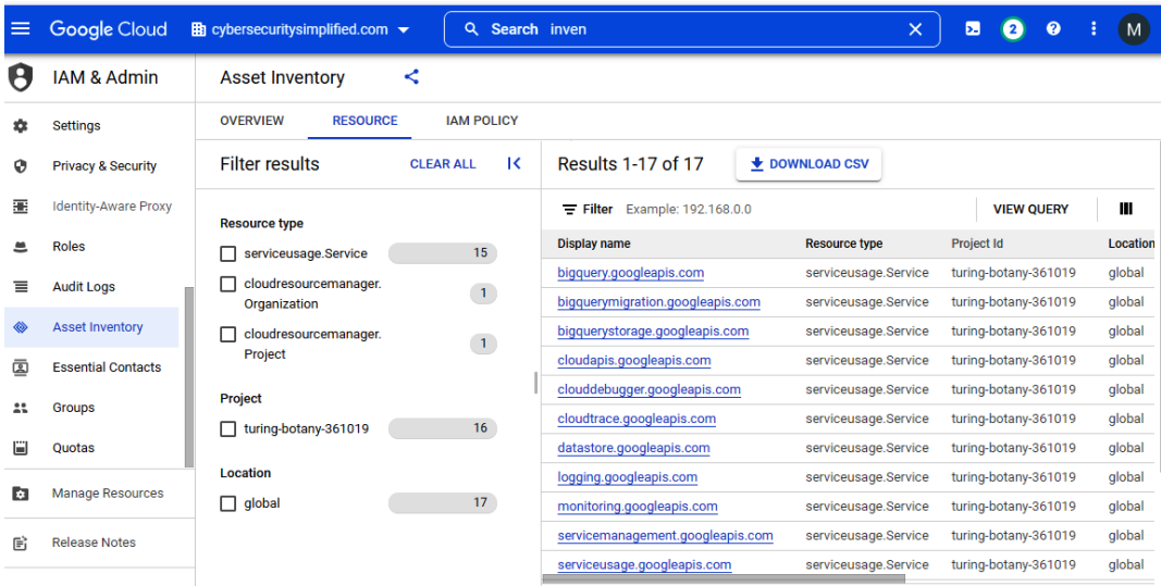
Figure 6.40 – The Asset Inventory RESOURCES tab
