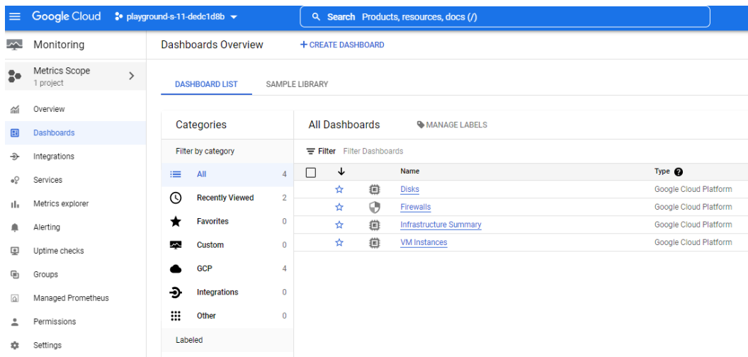
Figure 10.35 – Google Cloud Monitoring
