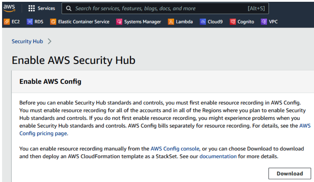
Figure 6.4 – Enabling AWS Config
