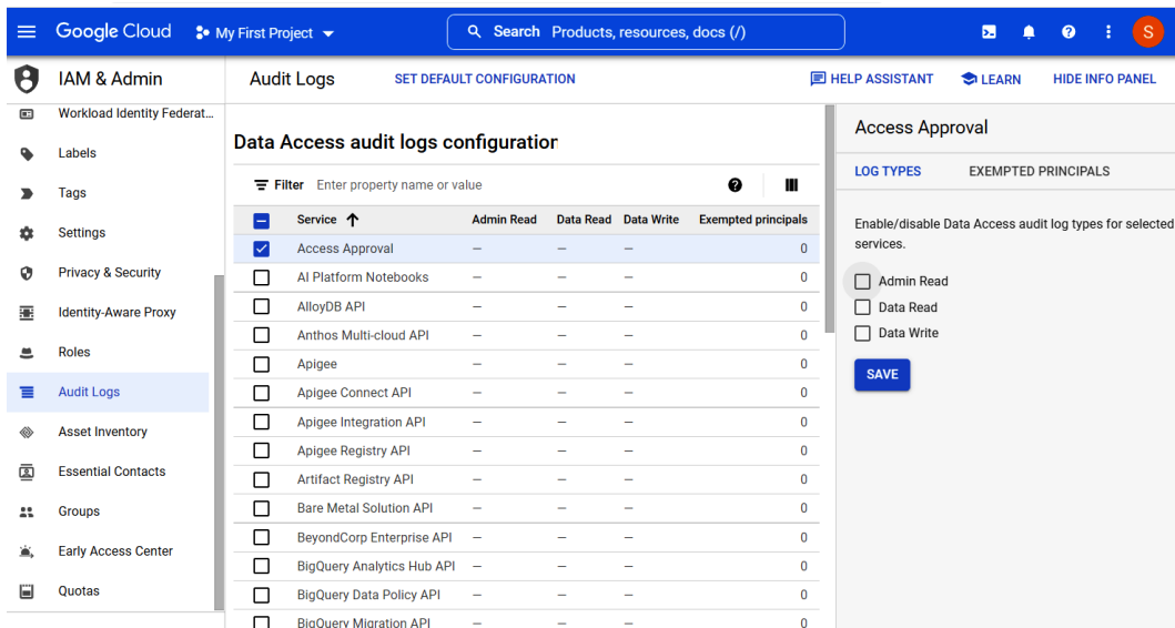
Figure 5.14 – Google Cloud audit log configuration
