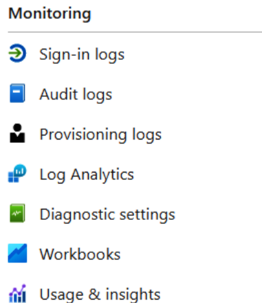
Figure 5.11 – Azure Monitoring
