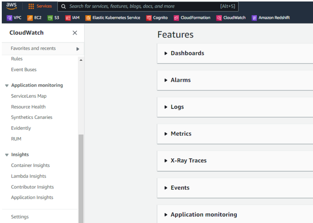
Figure 10.24 – Amazon CloudWatch
