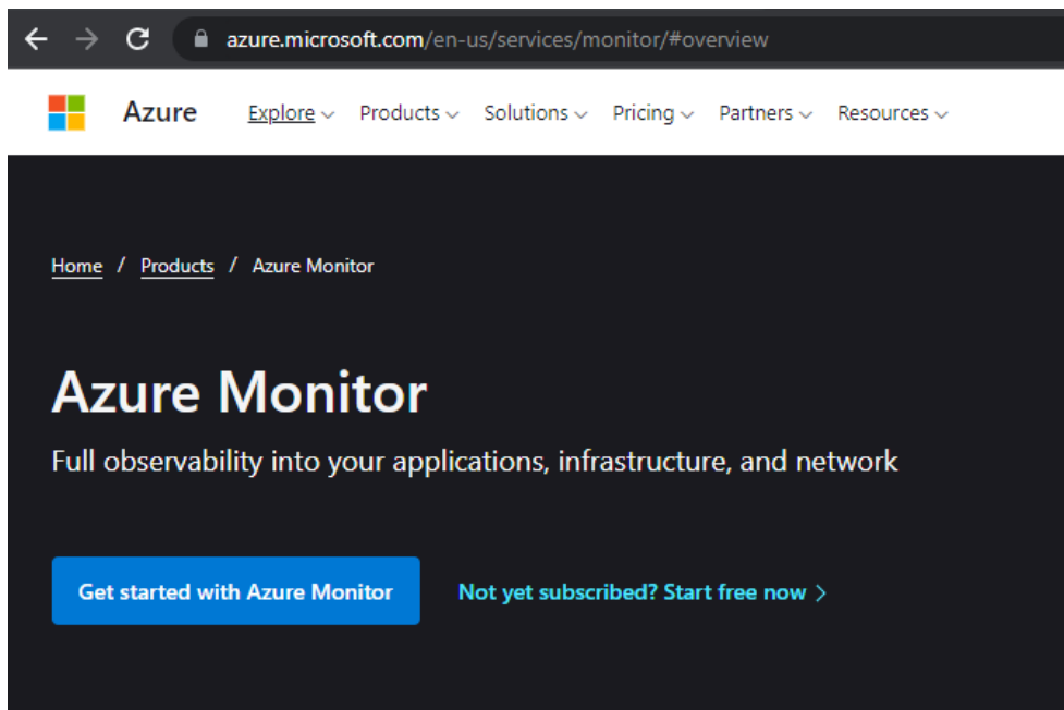
Figure 7.16 – Azure Monitor
