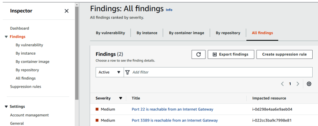
Figure 7.14 – The Amazon Inspector findings
