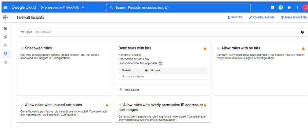
Figure 7.30 – Firewall Insights
