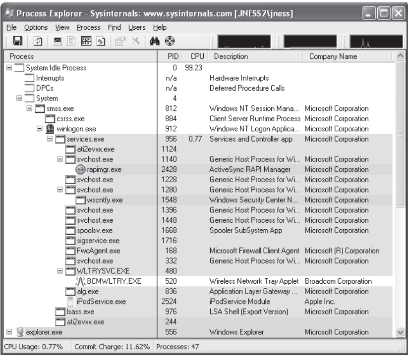
Figure 14-8 Process Explorer
