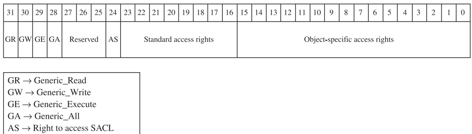
Figure 14-5 Access mask
