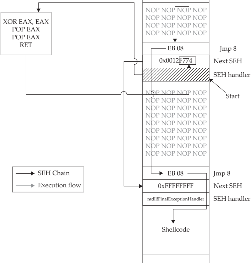
Figure 13-2 Sysdream.com technique to bypass SEHOP (used with permission)
