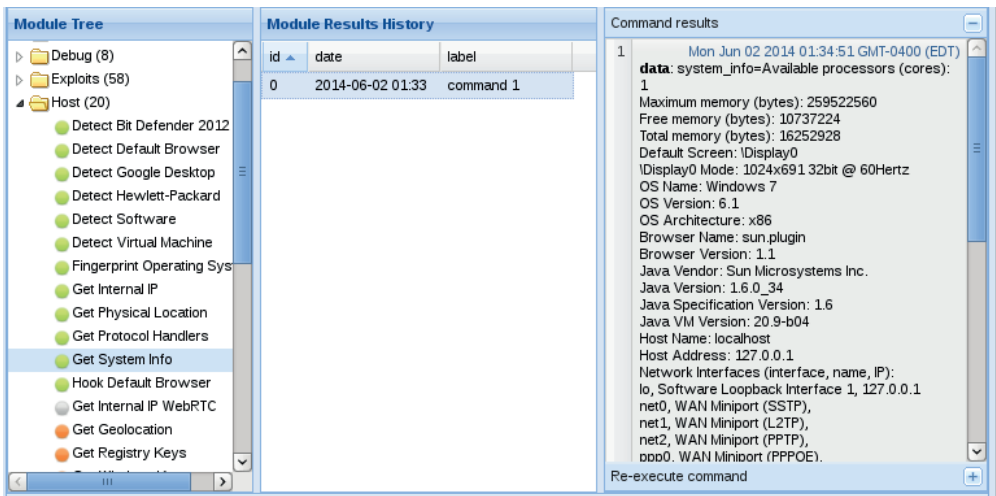
Figure 18-12 The output from the Get System Info module
