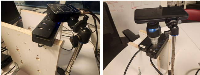
Fig. 3. Recovering a frequency scan using a photodiode (left) and a smartphone (right), by capturing video footage of the power LED of a USB hub.
