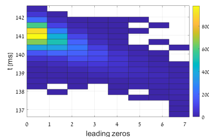
Fig. 9. A heat map of the estimated execution times of 7,826 ECDSA signature operations as a function of the number of leading zero bits in the nonce.
