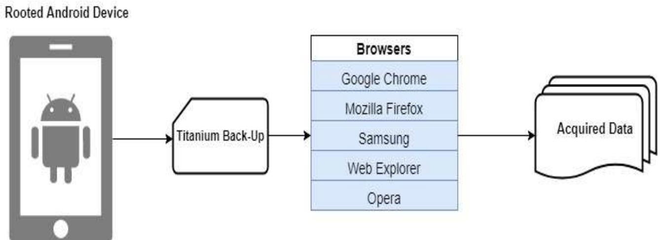
Figure 2. Collection of local storage
