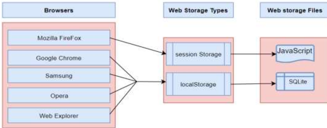
Figure 2. Web Storage Implementation on Android Platform
