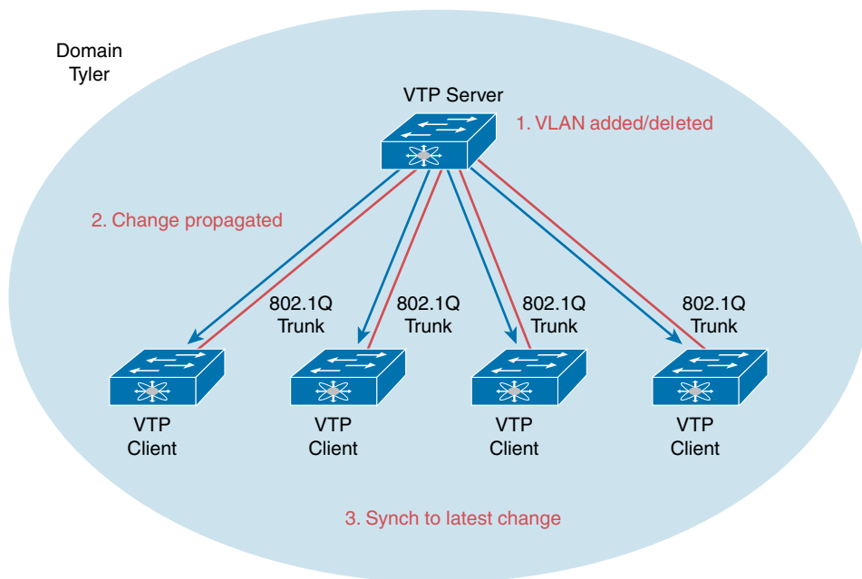
Figure 7-3 VTP Operation
