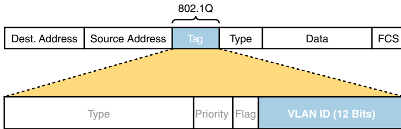
Figure 6-6 802.1Q Trunking
