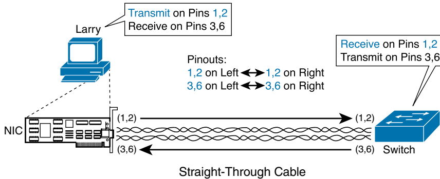
Figure 3-12 Ethernet Strait-Through Cable Concept
