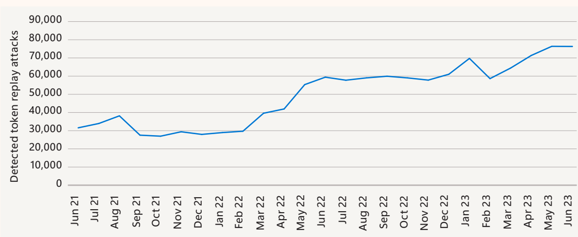
Token replay attacks consistently growing since early 2022
