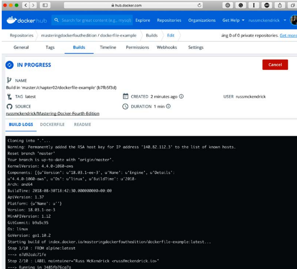
Figure 3.14 – Viewing the progress of the build
