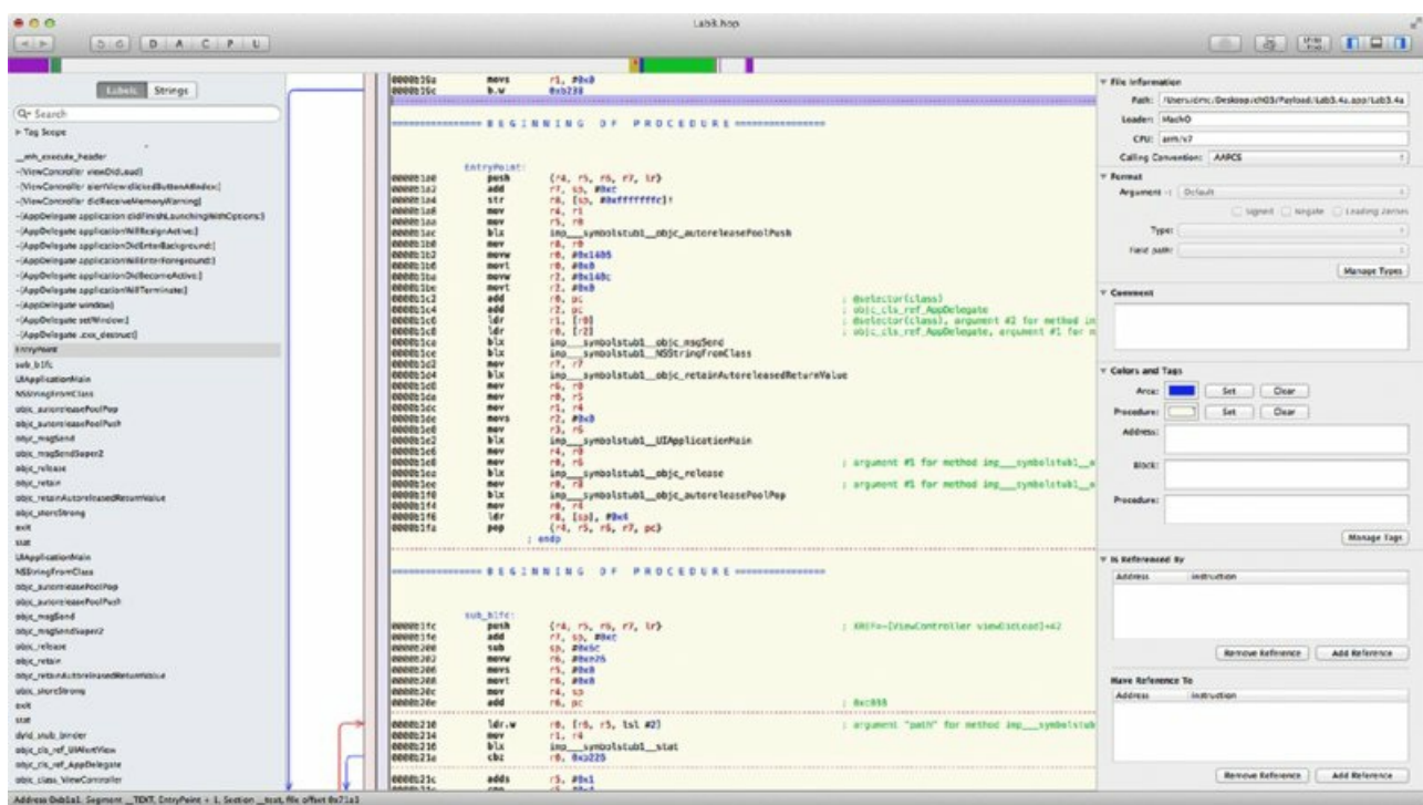
Figure 3.8 Hopper disassembler
