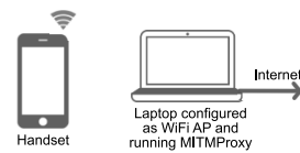
Fig. 1. Measurement setup. The mobile handset is configured to access the internet using a WiFi access point hosted on a laptop, use of cellular/mobile data is disabled. The laptop also has a wired internet connection. When an app on the handset starts a new network connection the laptop pretends to be the destination server so that it can decrypt the traffic. It then creates an onward connection to the actual target server and acts as an intermediary relaying requests and their replies between the handset app and the target server while logging the traffic.
