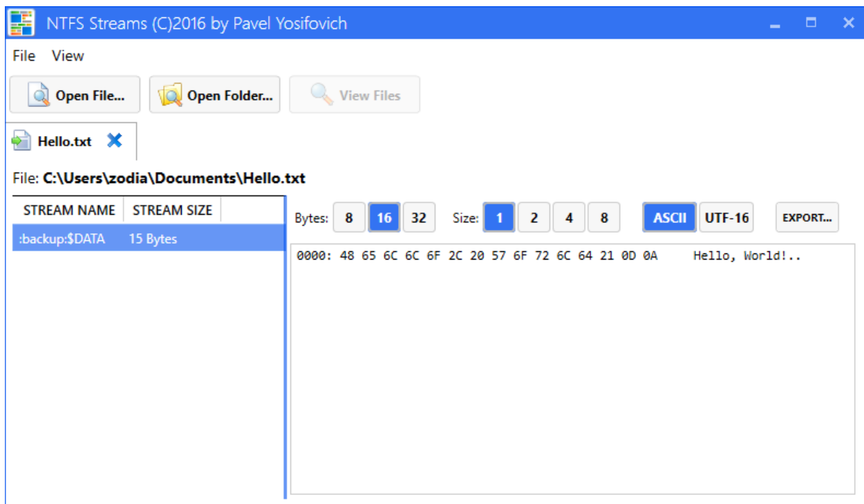
Figure 10-11: NtfsStreams with a file backup
