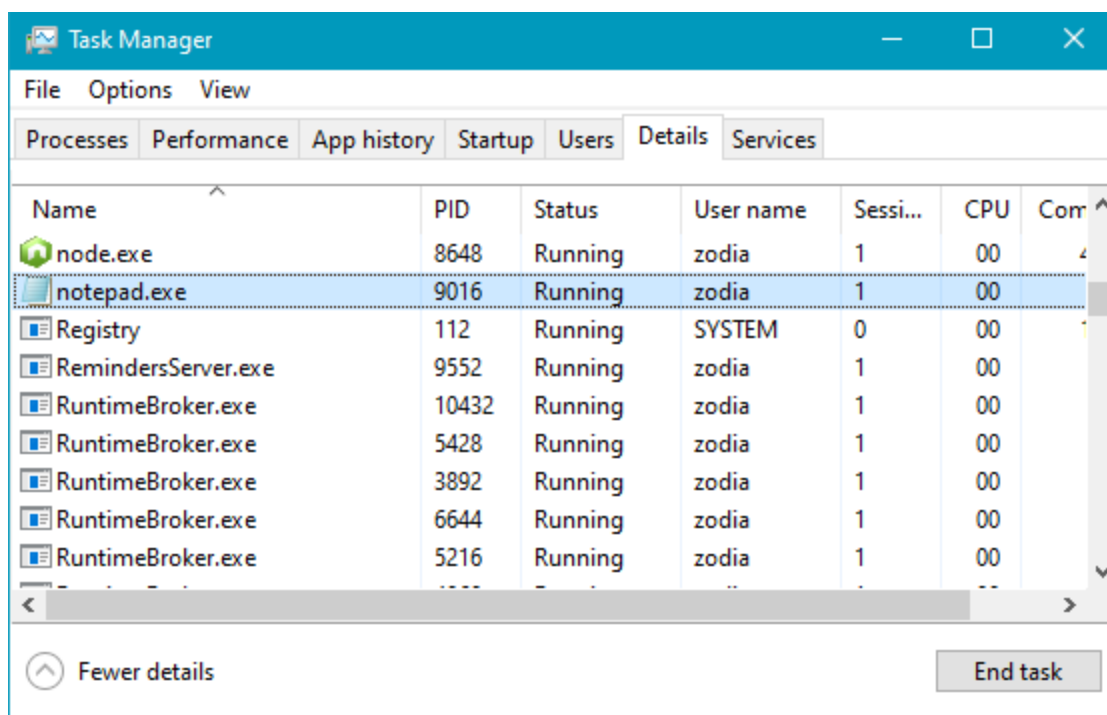
Figure 9-1: Notepad running
