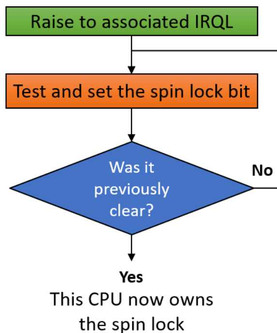
Figure 6-12: Acquiring a Spin Lock
