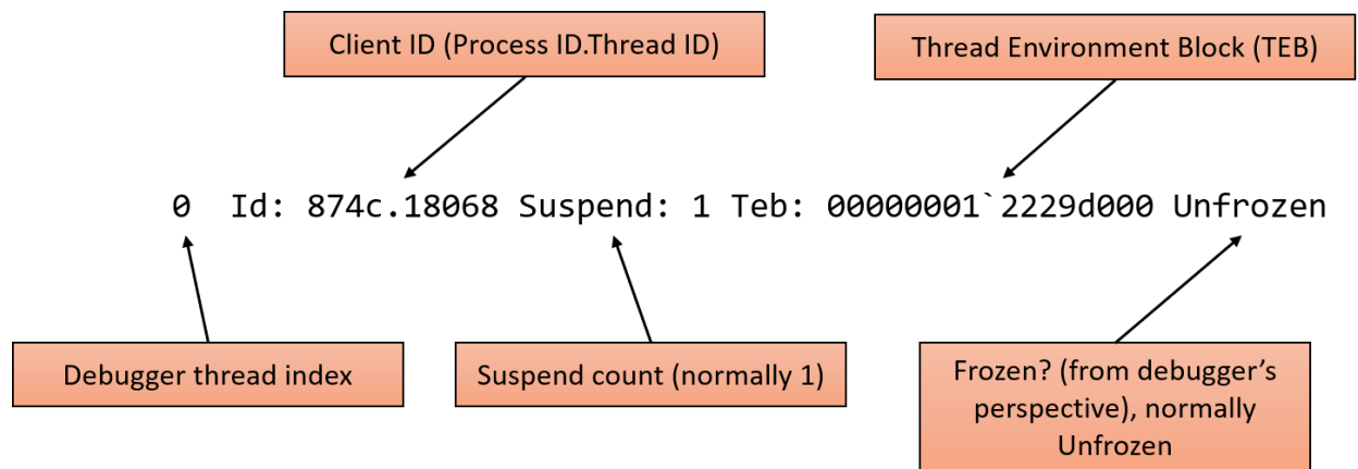
Figure 5-4: Thread information for the ~ command
