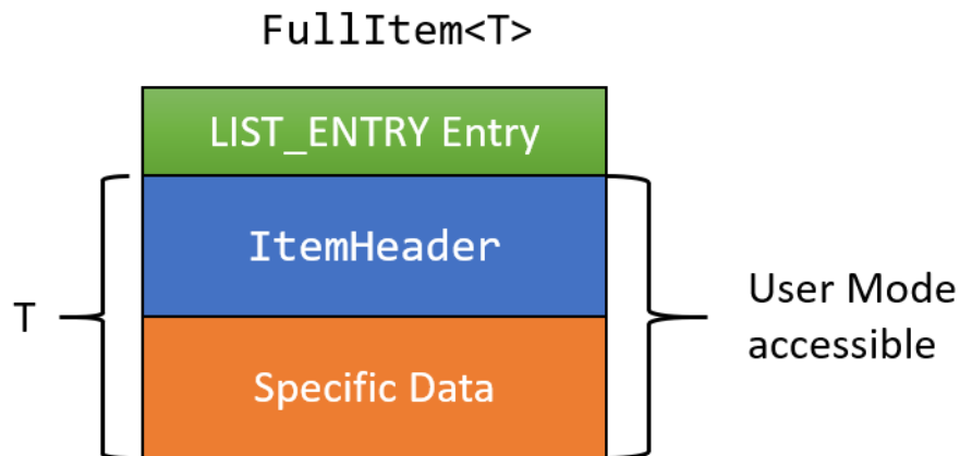
Figure 8-2: FullItem<T> layout
