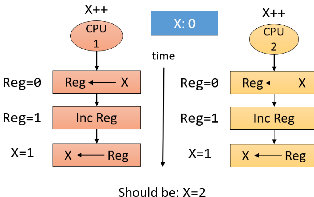
Figure 6-9: Concurrent increment
