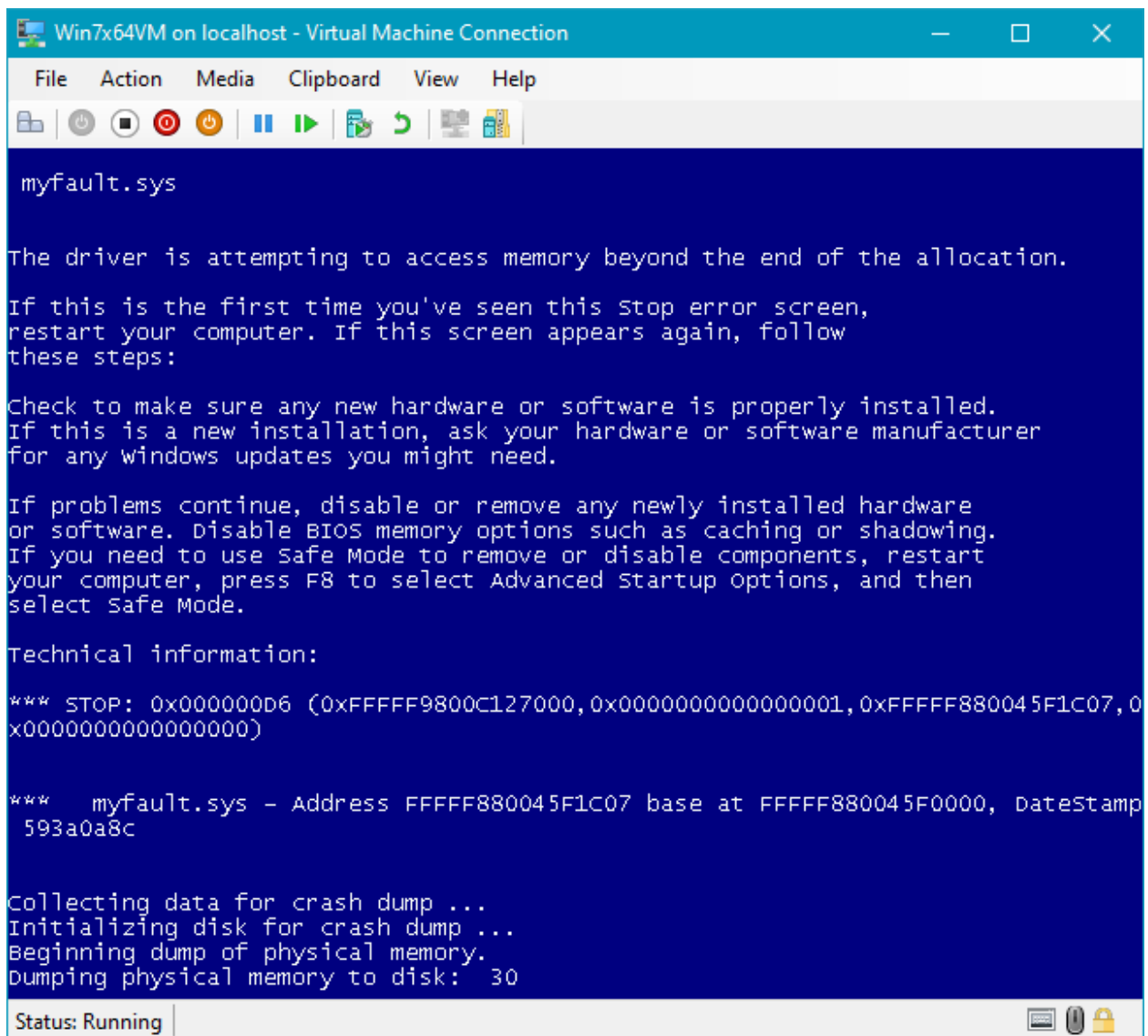
Figure 11-11: NotMyFault BSOD on Windows 7 with Buffer overflow and Verifier active
