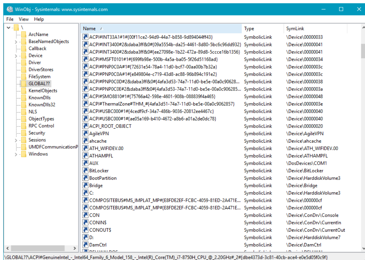
Figure 3-3: Symbolic links directory in WinObj
