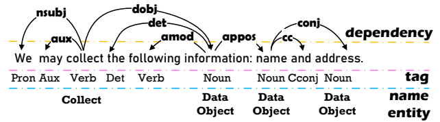
Figure 1: Sentence parsing
