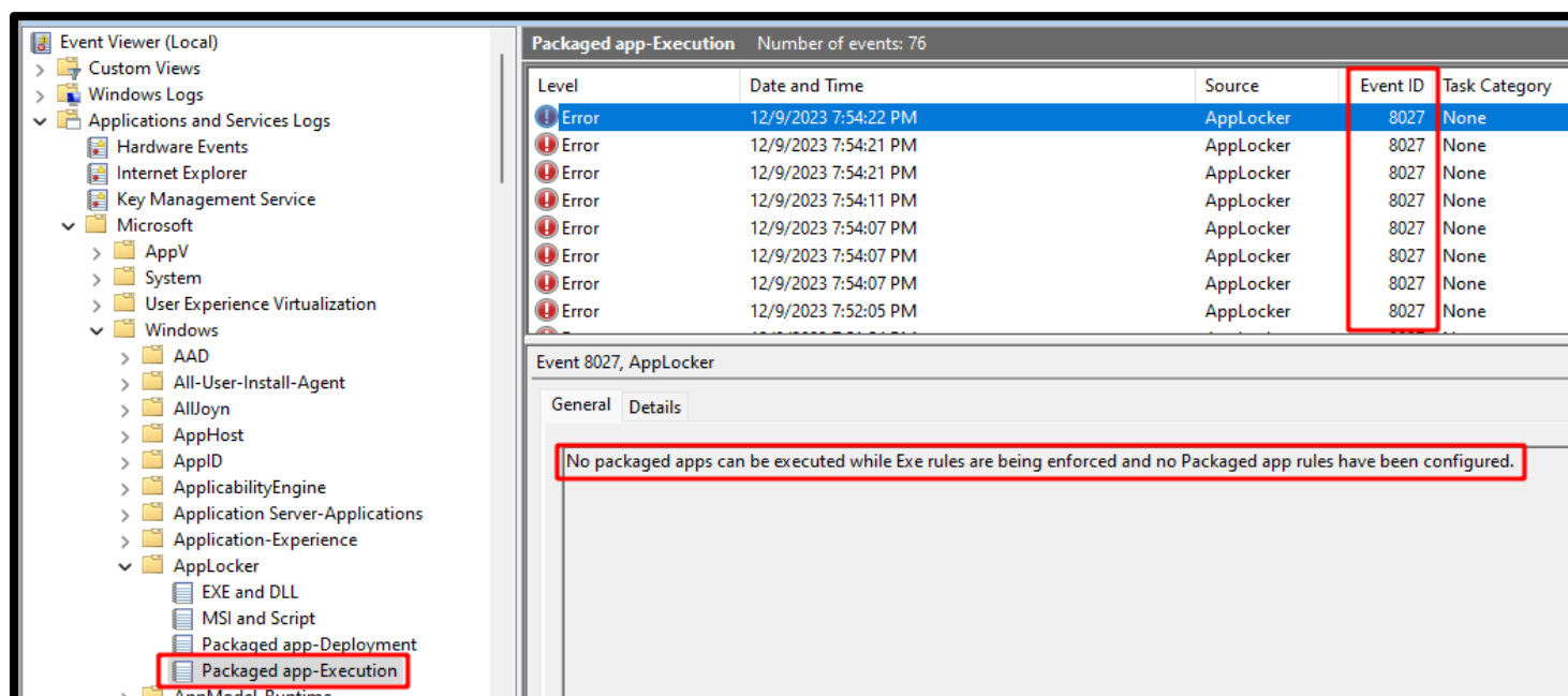
Figure 5. Event ID 8027 Blocking Execution of Default Windows Applications
