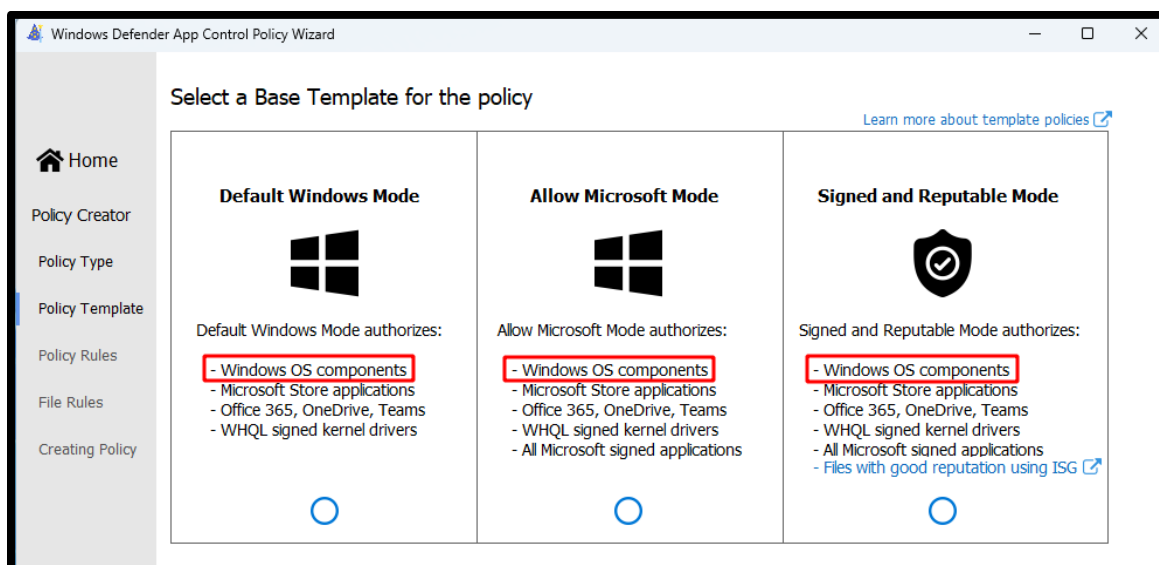
Figure 1. WDAC Default Policies Inherently Trust All Windows OS Binaries
