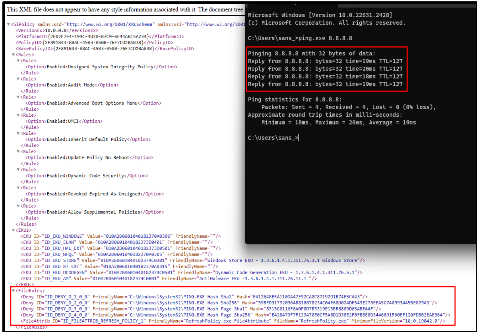
Figure 2. WDAC Default Windows Mode Policy with Ping.EXE Deny Rule Still Allowing Ping.exe Execution
