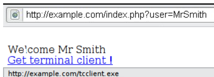
Figure 4.7.1-1: XSS Example 1
