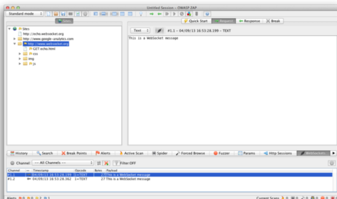
Figure 4.11.10-1: ZAP WebSockets
