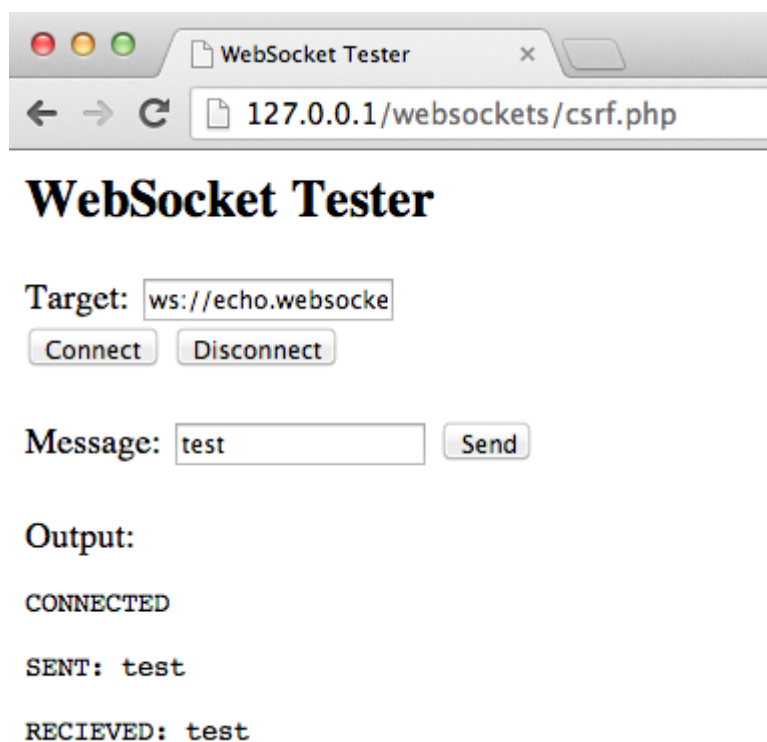
Figure 4.11.10-2: WebSocket Client
