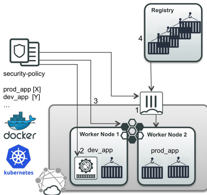
Figure 11: Container security.
