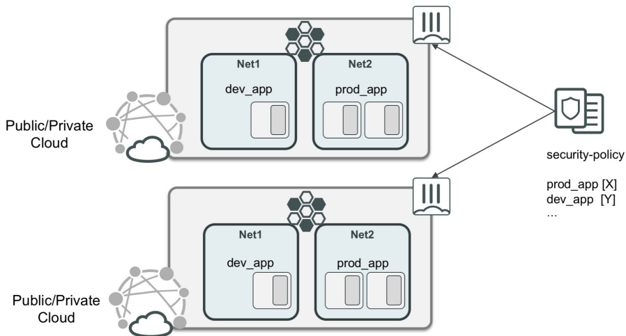
Figure 10: Logical segmentation.
