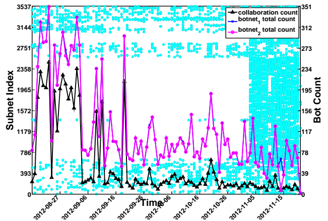
Figure 3: Intra-family collaboration for Blackenergy
