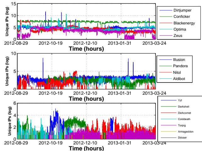
Figure 1: Botnet stability of three groups (based on botnet size)
