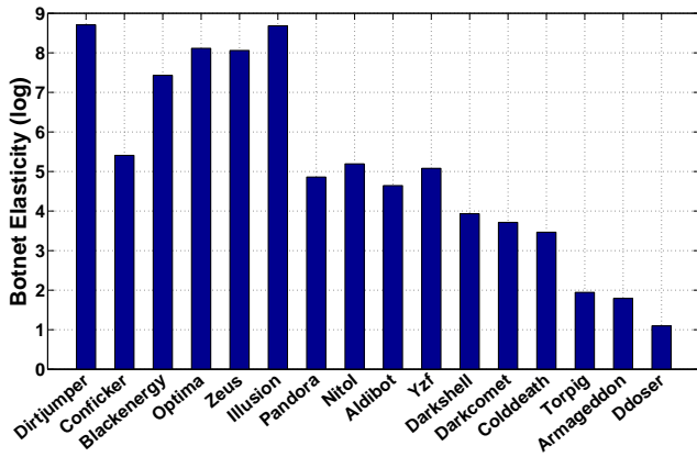
Figure 2: Botnet Elasticity
