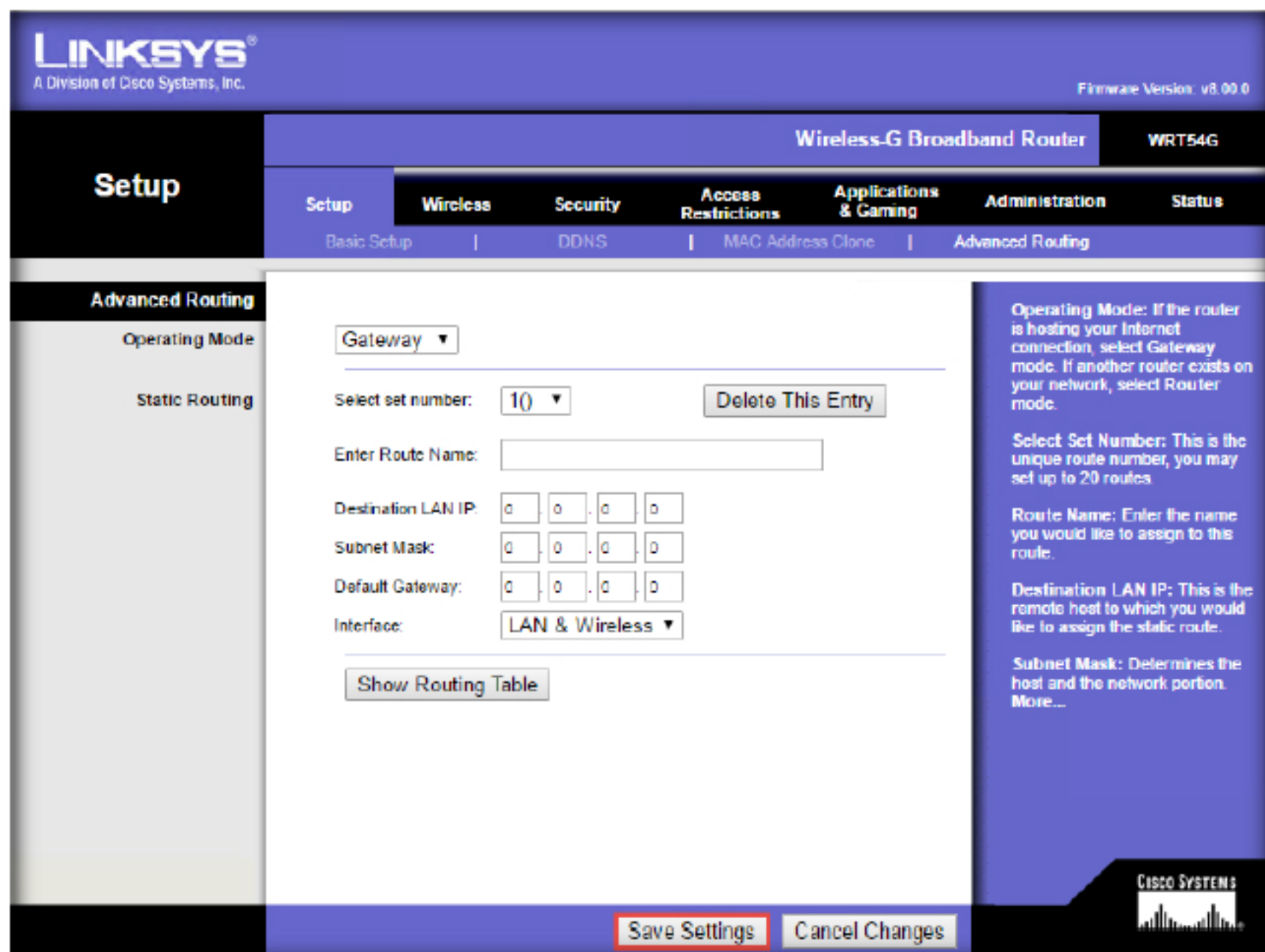
FIGURE 1.26 save Settings
