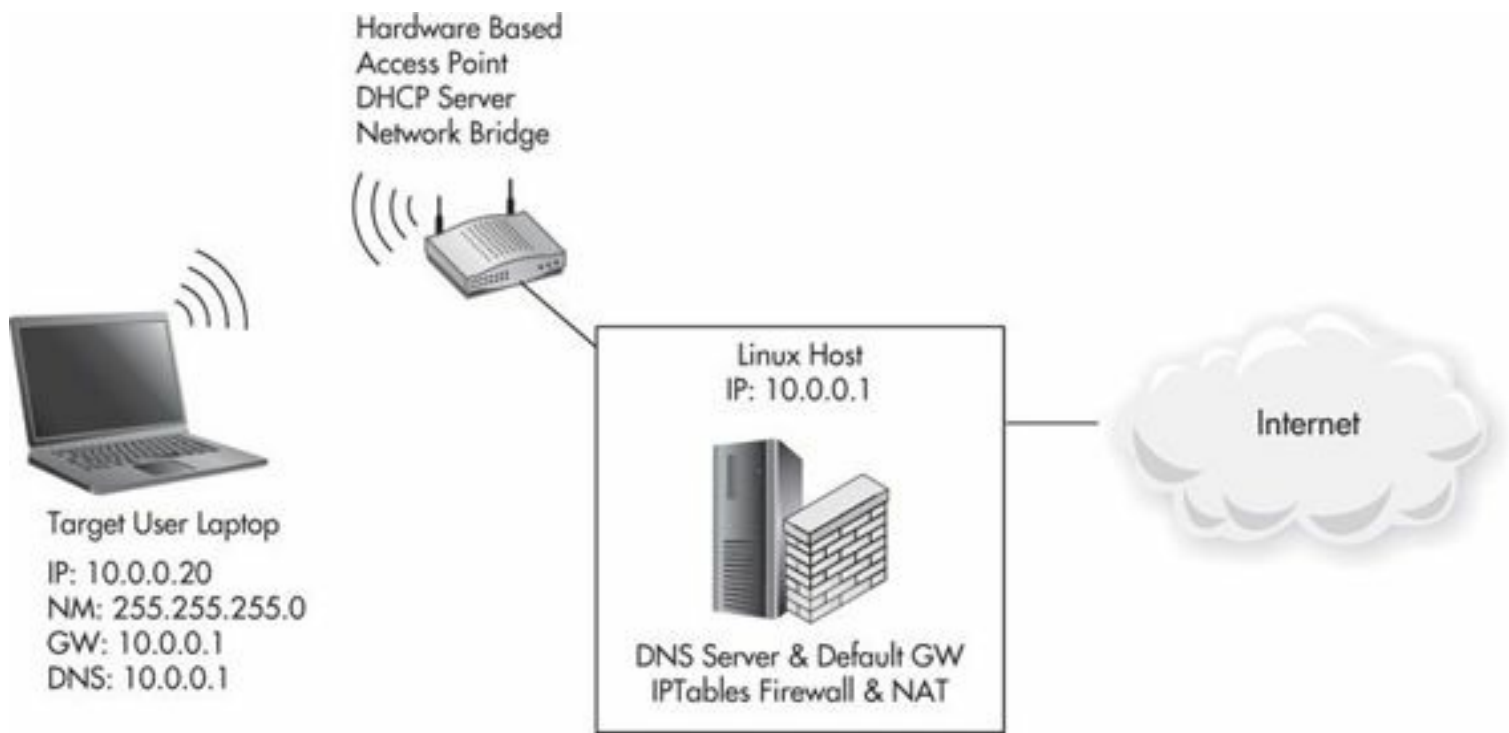
Figure 7-17 Using the hardware access point and Linux gateway system
