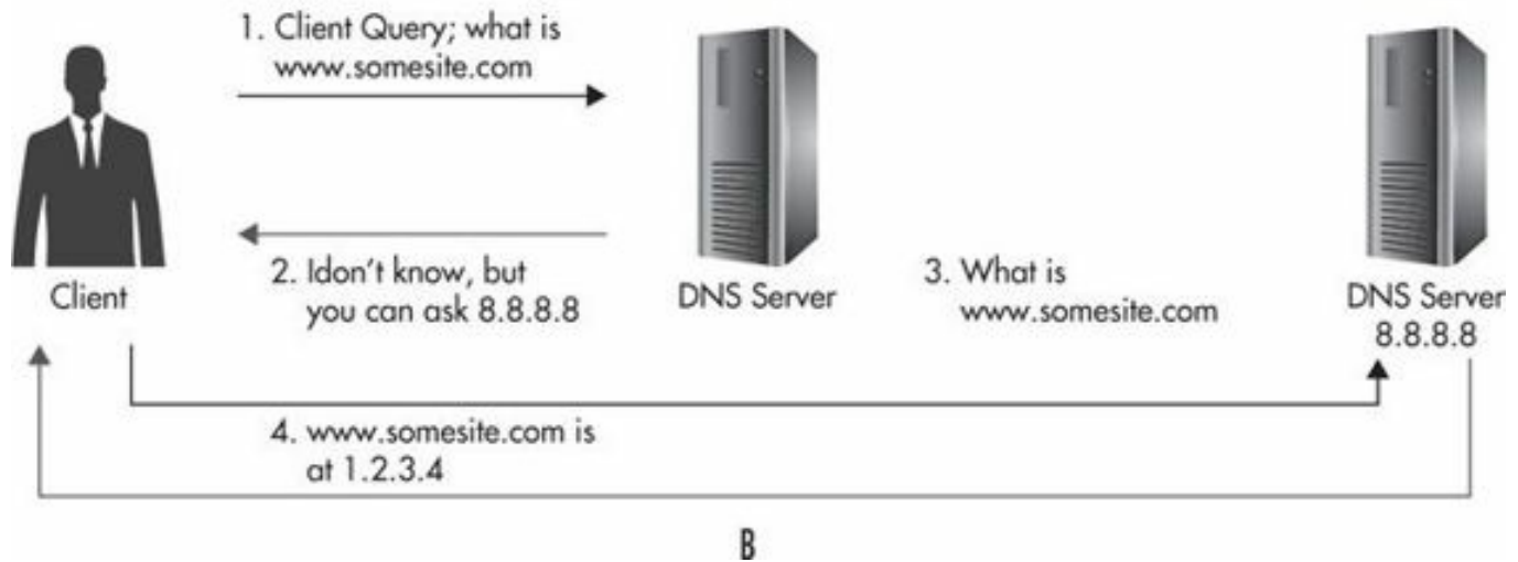
Figure 4-4 Recursive and iterative DNS queries
