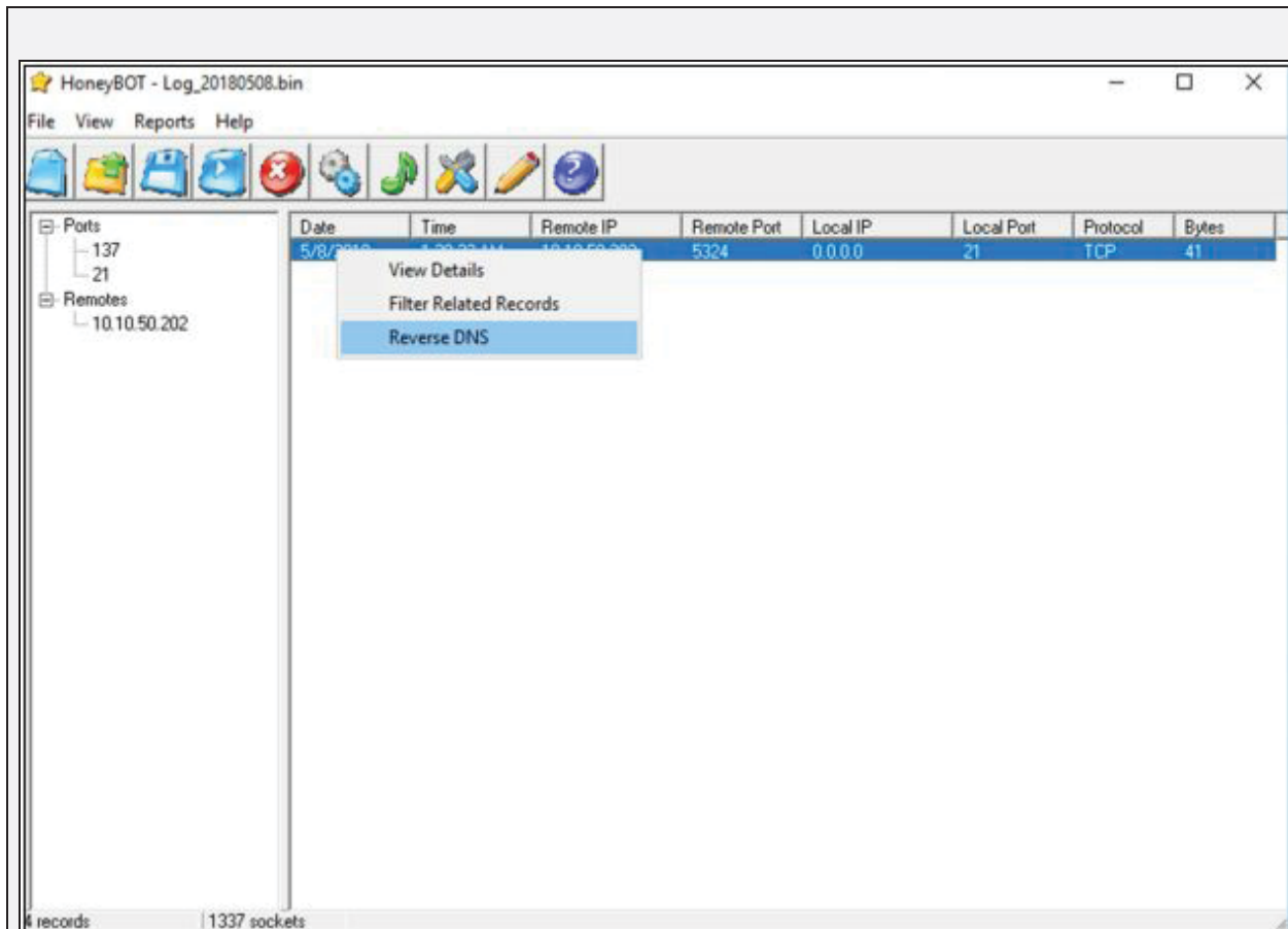
Figure 12-16. Reverse DNS
