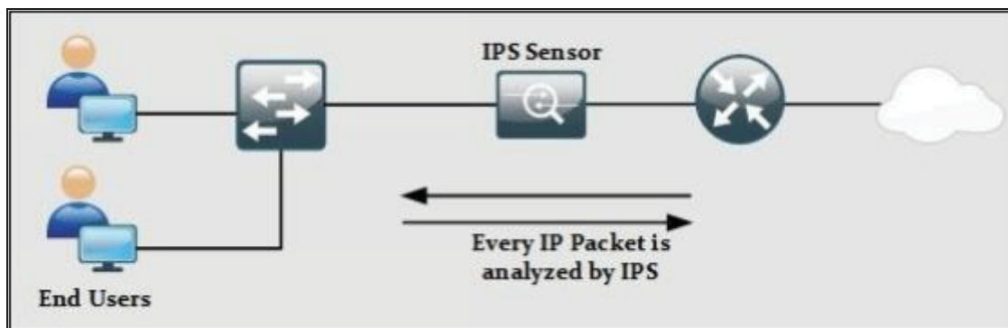
Figure 12-01. In-line Deployment of IPS Sensor
