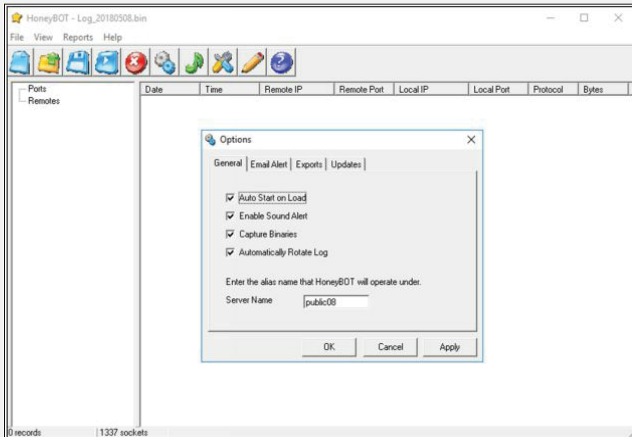
Figure 12-10. HoneyBot Application
