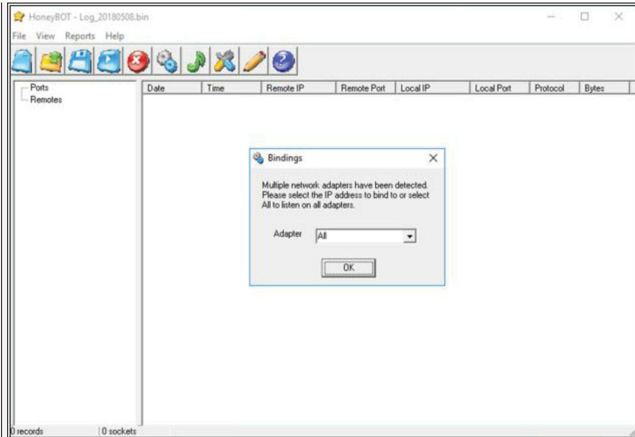
Figure 12-11. HoneyBot Application
