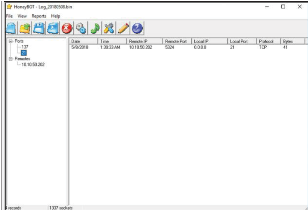
Figure 12-14. logs
