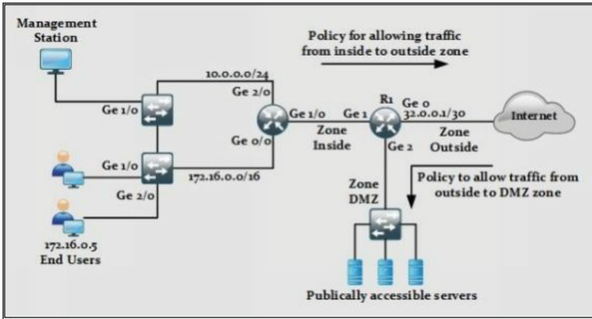
Figure 12-07. Cisco IOS Zone-Based Firewall Scenario
