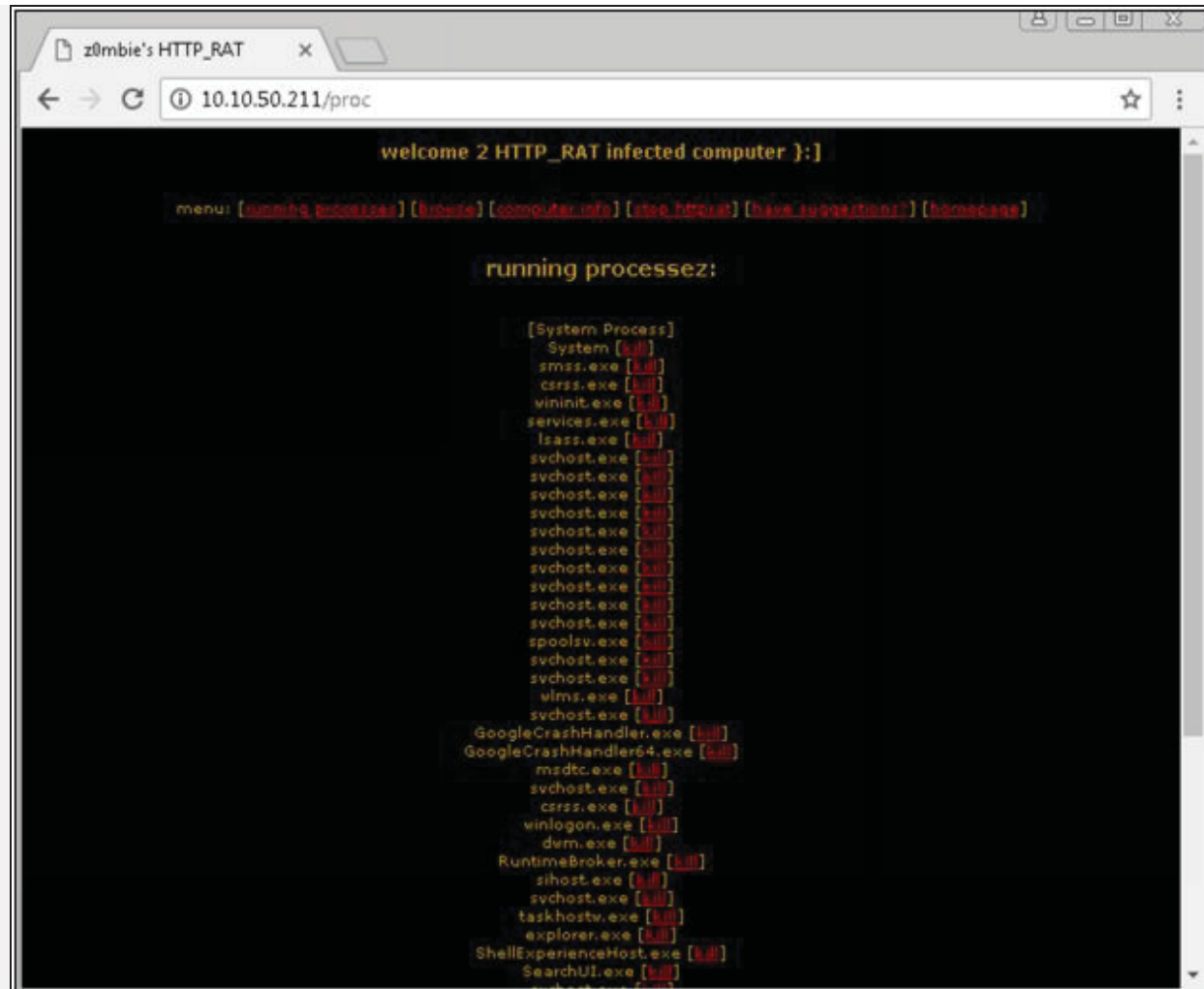
Figure 7-07 Running Process on Victim
