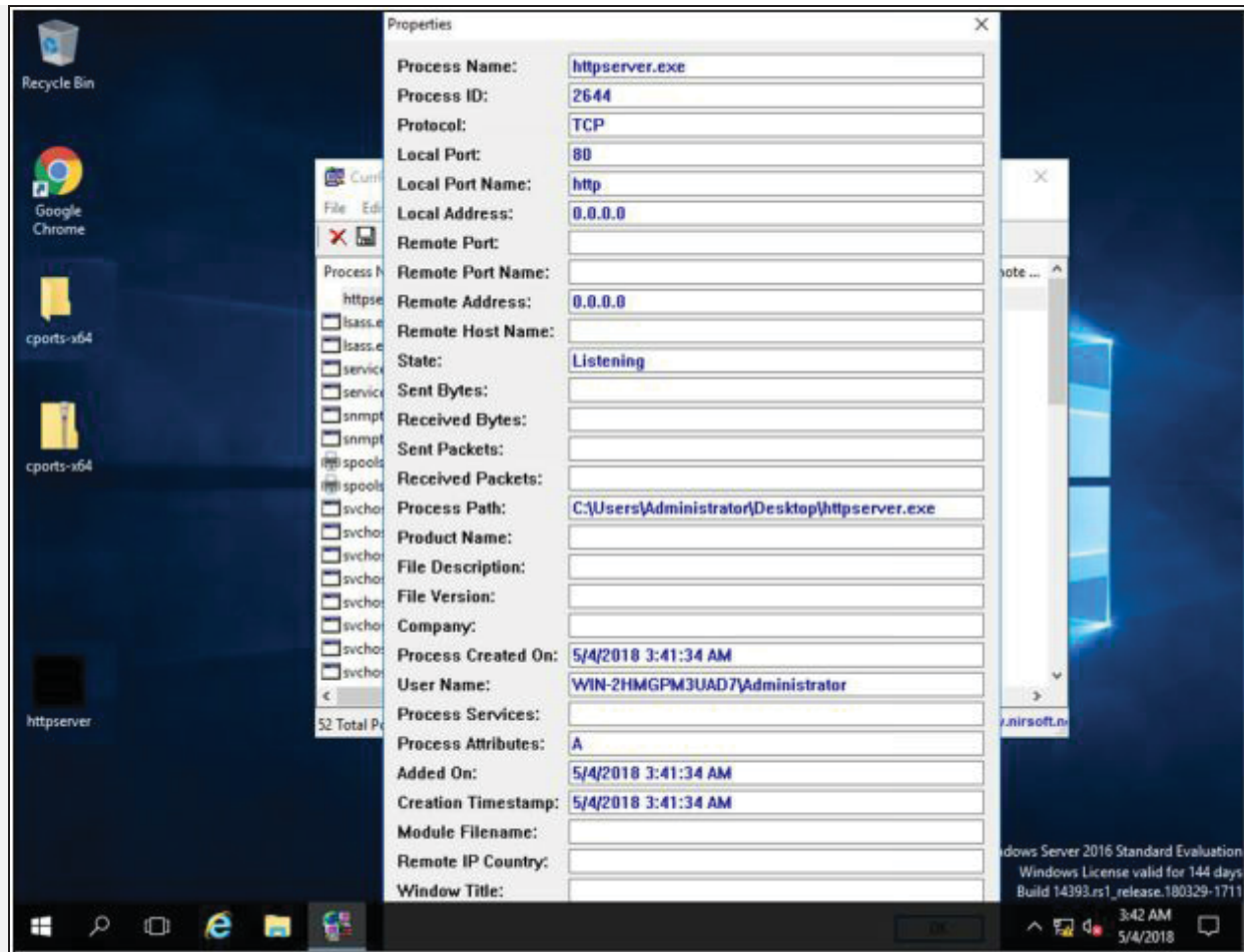
Figure 7-17 TCP connection properties
