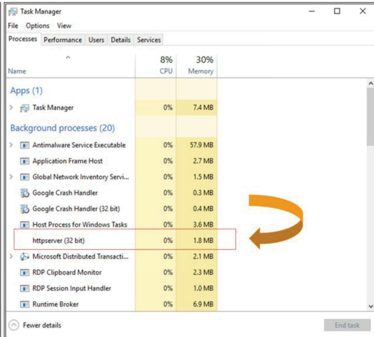
Figure 7-05 Trojan process on Victim machine
