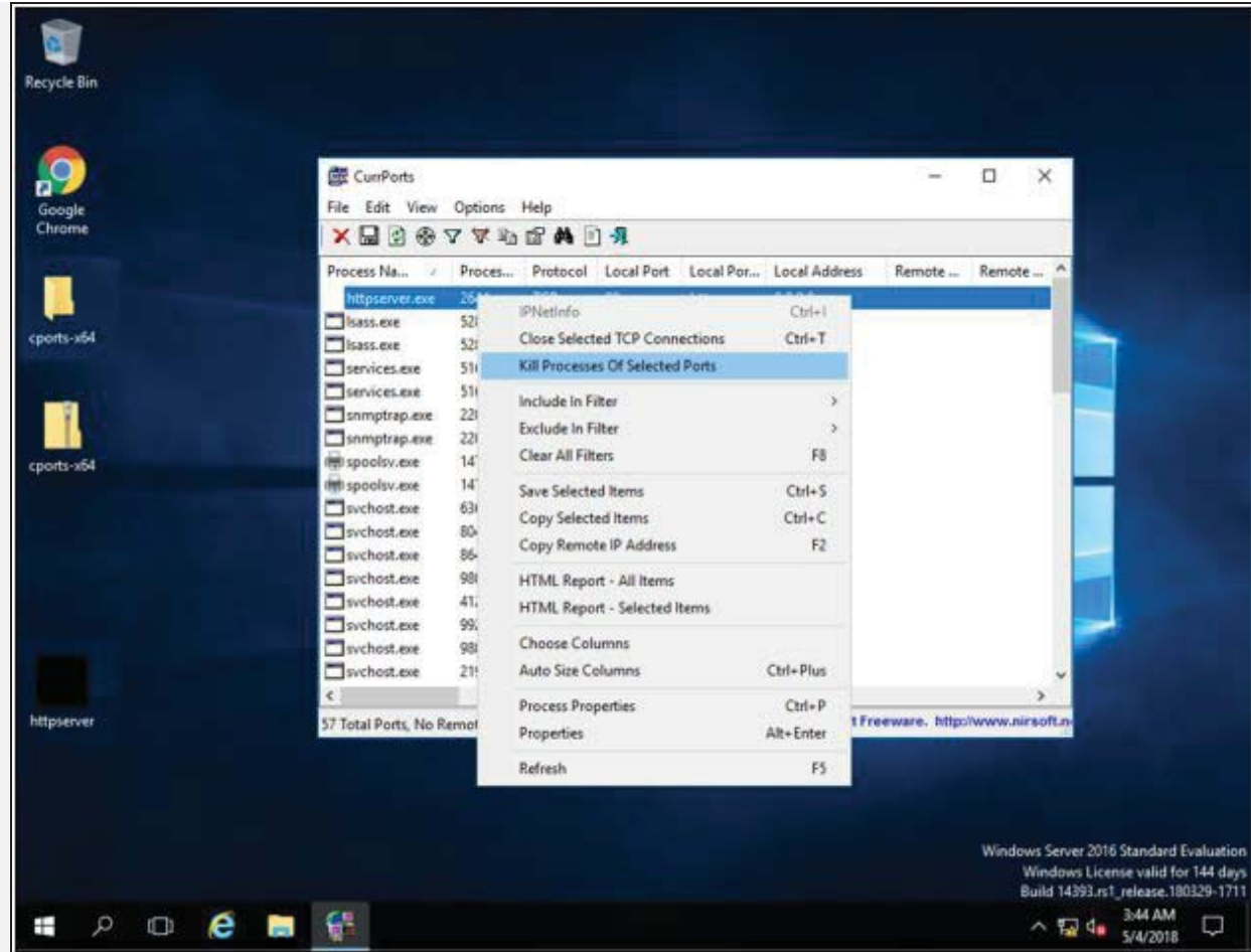
Figure 7-19 Killing TCP connection properties
