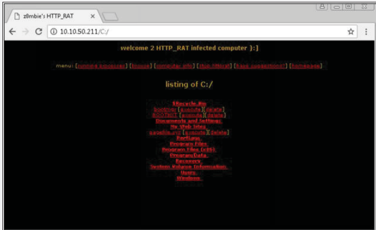
Figure 7-09 C drive of Victim
