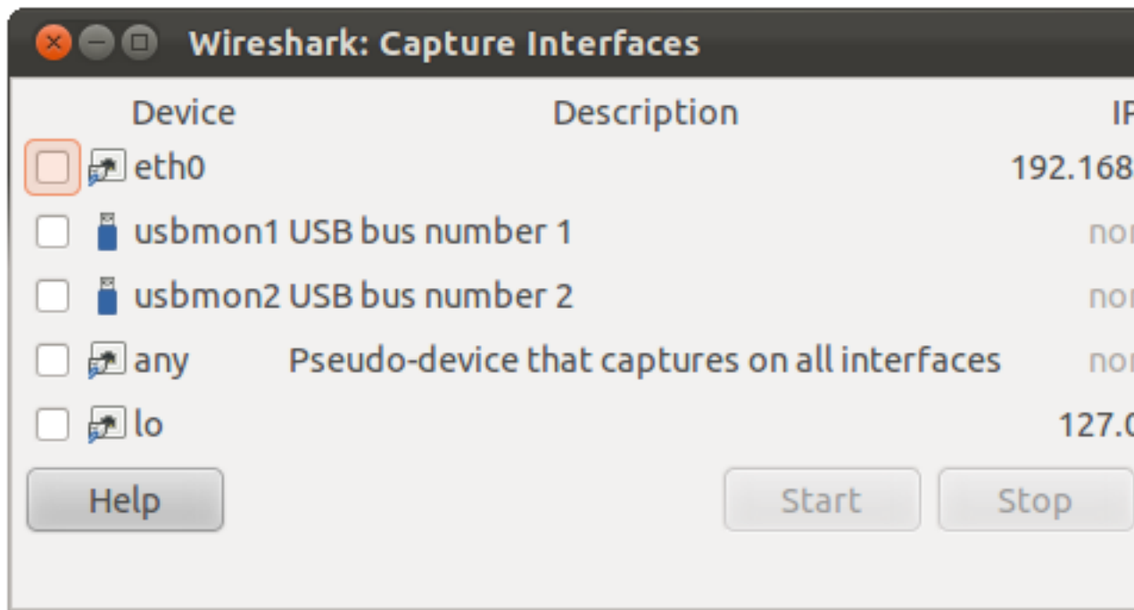
Figure 4.2. The "Capture Interfaces" dialog box on Unix/Linux
