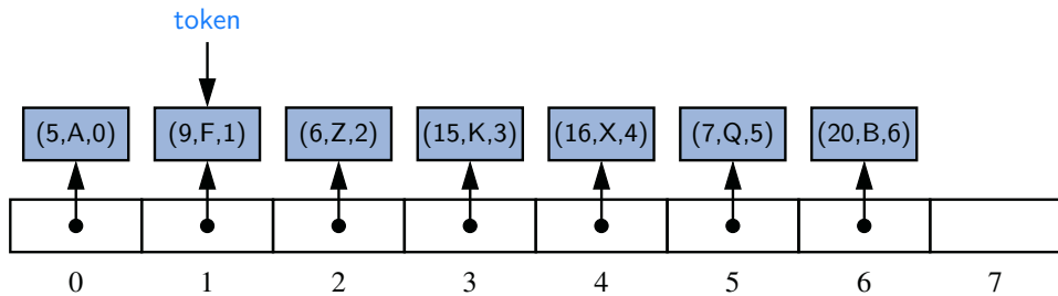
Figure 9.11: The result of a call to removeMin() on the heap originally portrayed in Figure 9.10. Identifier token continues to reference the same entry as in the original configuration, but the placement of that entry in the array has changed, as has the third field of the entry.
