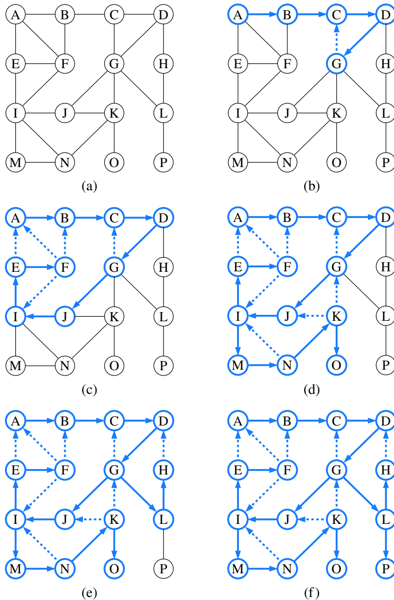
Figure 14.9: Example of depth-first search traversal on an undirected graph starting at vertex A . We assume that a vertex’s adjacencies are considered in alphabetical order. Visited vertices and explored edges are highlighted, with discovery edges drawn as solid lines and nontree (back) edges as dashed lines: (a) input graph; (b) path of tree edges, traced from A until back edge ( G,C ) is examined; (c) reaching F , which is a dead end; (d) after backtracking to I , resuming with edge ( I,M ), and hitting another dead end at O ; (e) after backtracking to G , continuing with edge ( G,L ), and hitting another dead end at H ; (f) final result.
