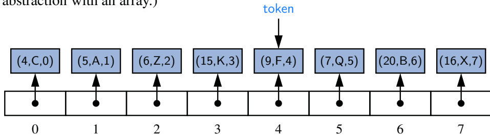
Figure 9.10: Representing a heap using an array of location-aware entries. The third field of each entry instance corresponds to the index of that entry within the array. Identifier token is presumed to be an entry reference in the user’s scope.
