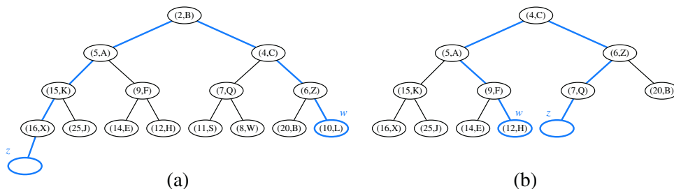
Figure 9.12: Two cases of updating the last node in a complete binary tree after operation insert or remove. Node w is the last node before operation insert or after operation remove. Node z is the last node after operation insert or before operation remove.
